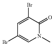
3,5-Dibromo-1-methyl-1H-pyridin-2-one (1)
