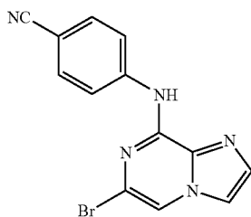
4-(6-Bromo-imidazo[1,2-a]pyrazin-8-ylamino)-benzonitrile
