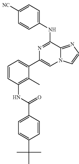
4-tert-Butyl-N-{3-[8-(4-cyano-phenylamino)-imidazo[1,2-a]pyrazin-6-yl]-2-methyl-phenyl}-benzamide
