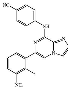
4-[6-(3-Amino-2-methyl-phenyl)-imidazo[1,2-a]pyrazin-8-ylamino]-benzonitrile
