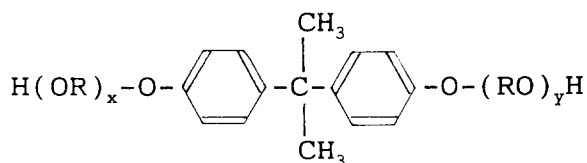
Formula (II)
