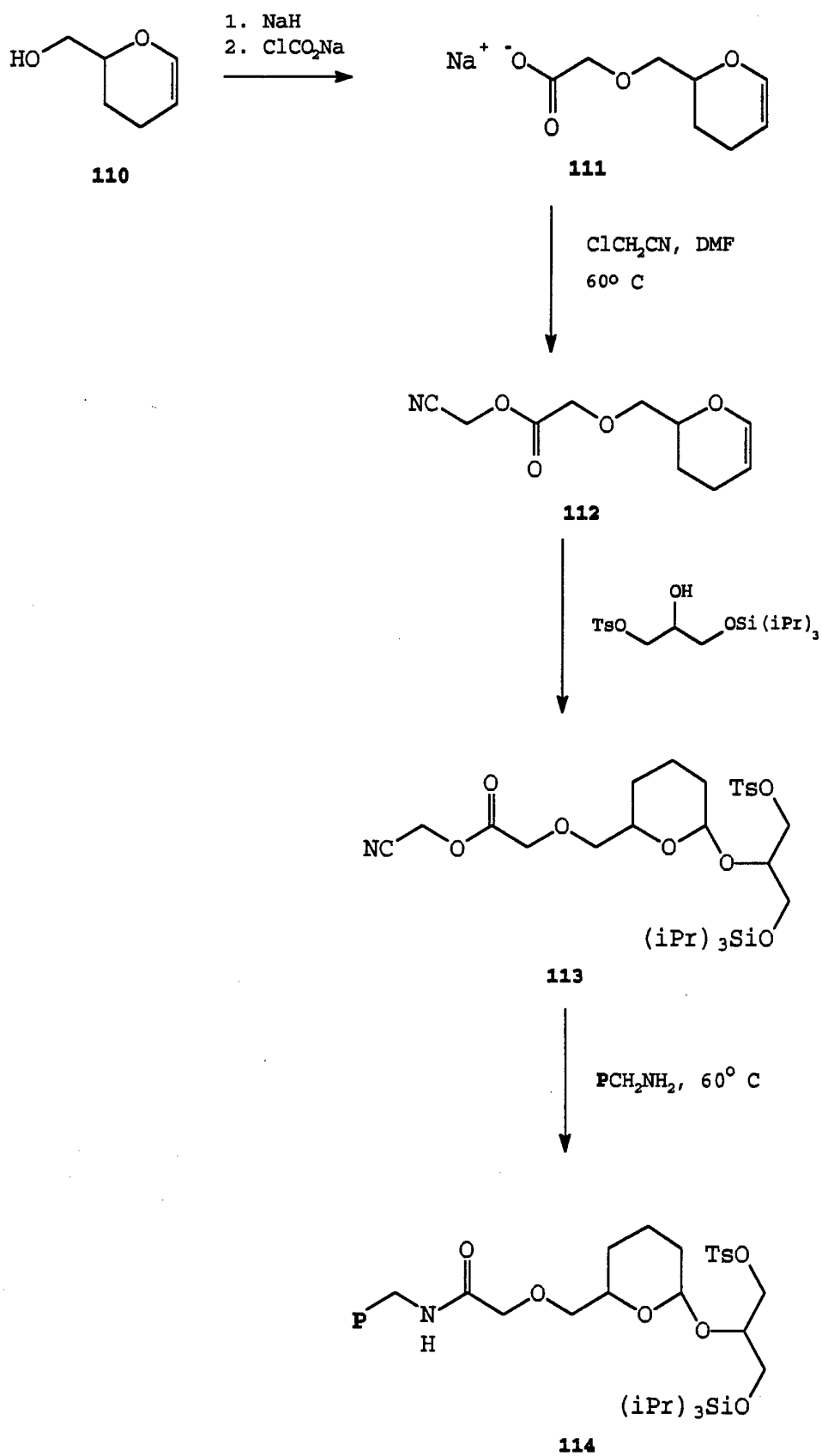
REACTION SCHEME XVIIIA
