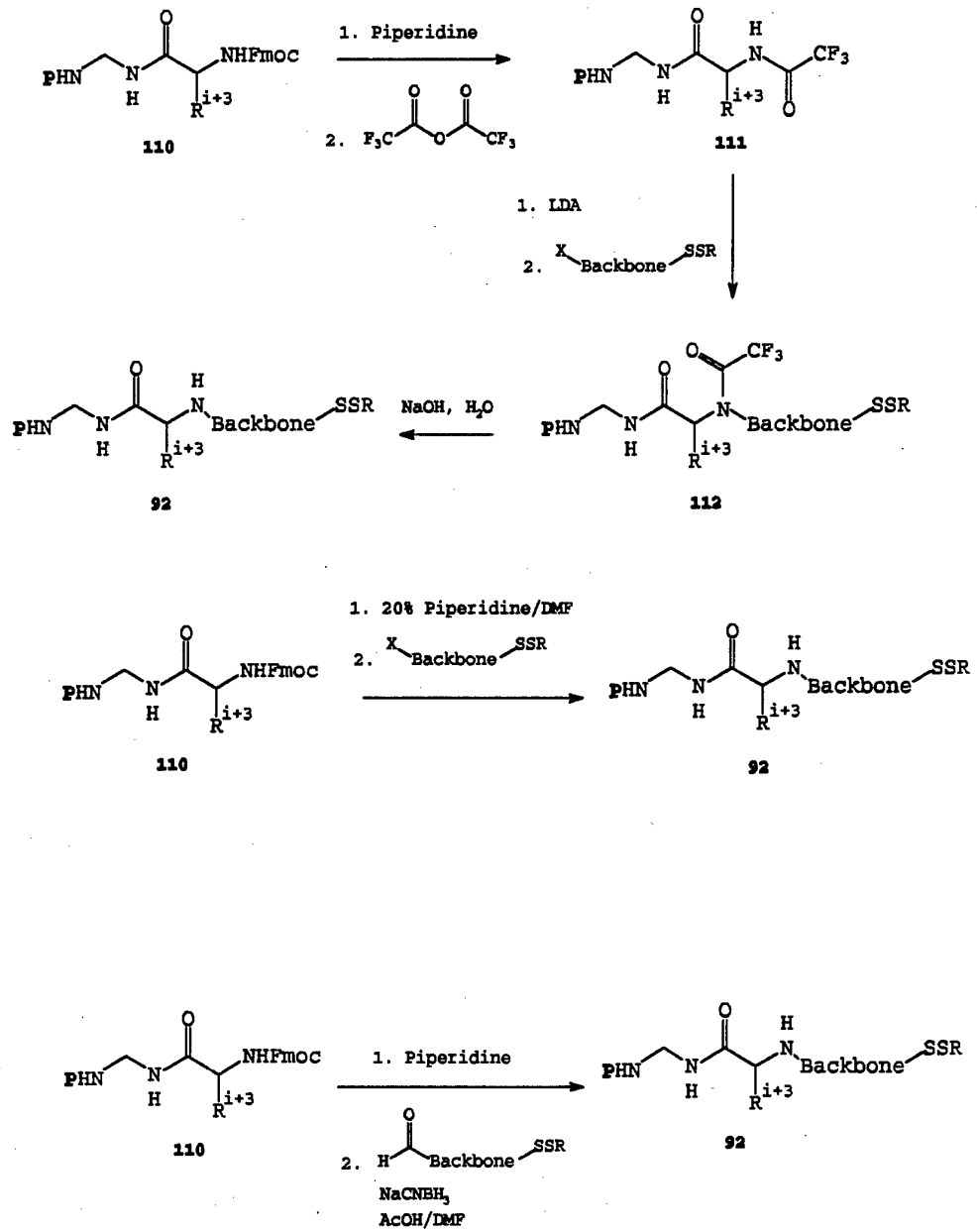
REACTION SCHEME XVI
