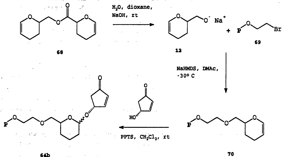
REACTION SCHEME X
