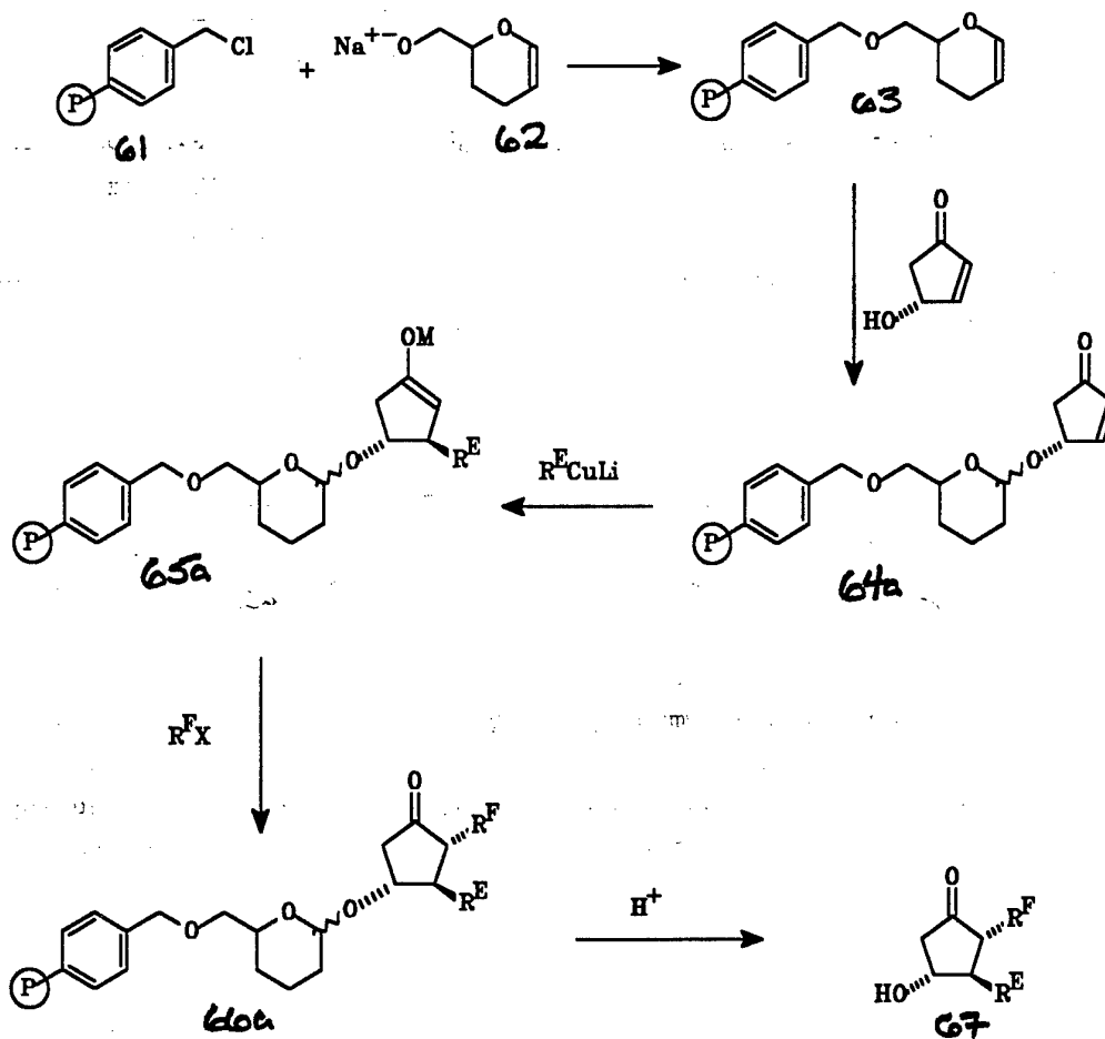
REACTION SCHEME IX
