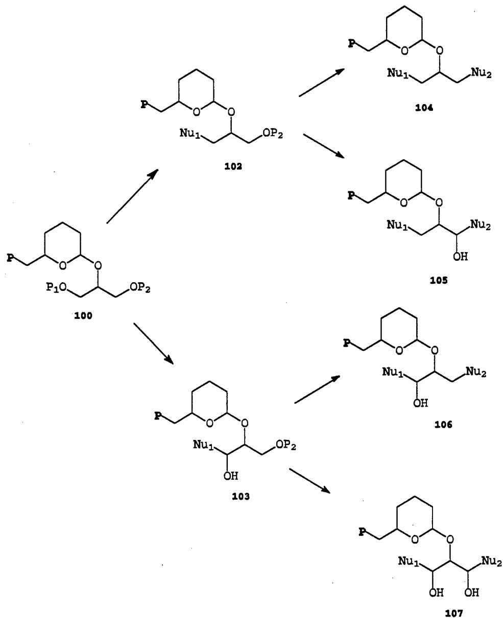
REACTION SCHEME XVII
