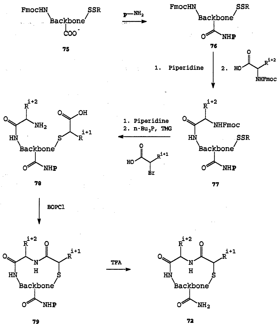
REACTION SCHEME XIII
