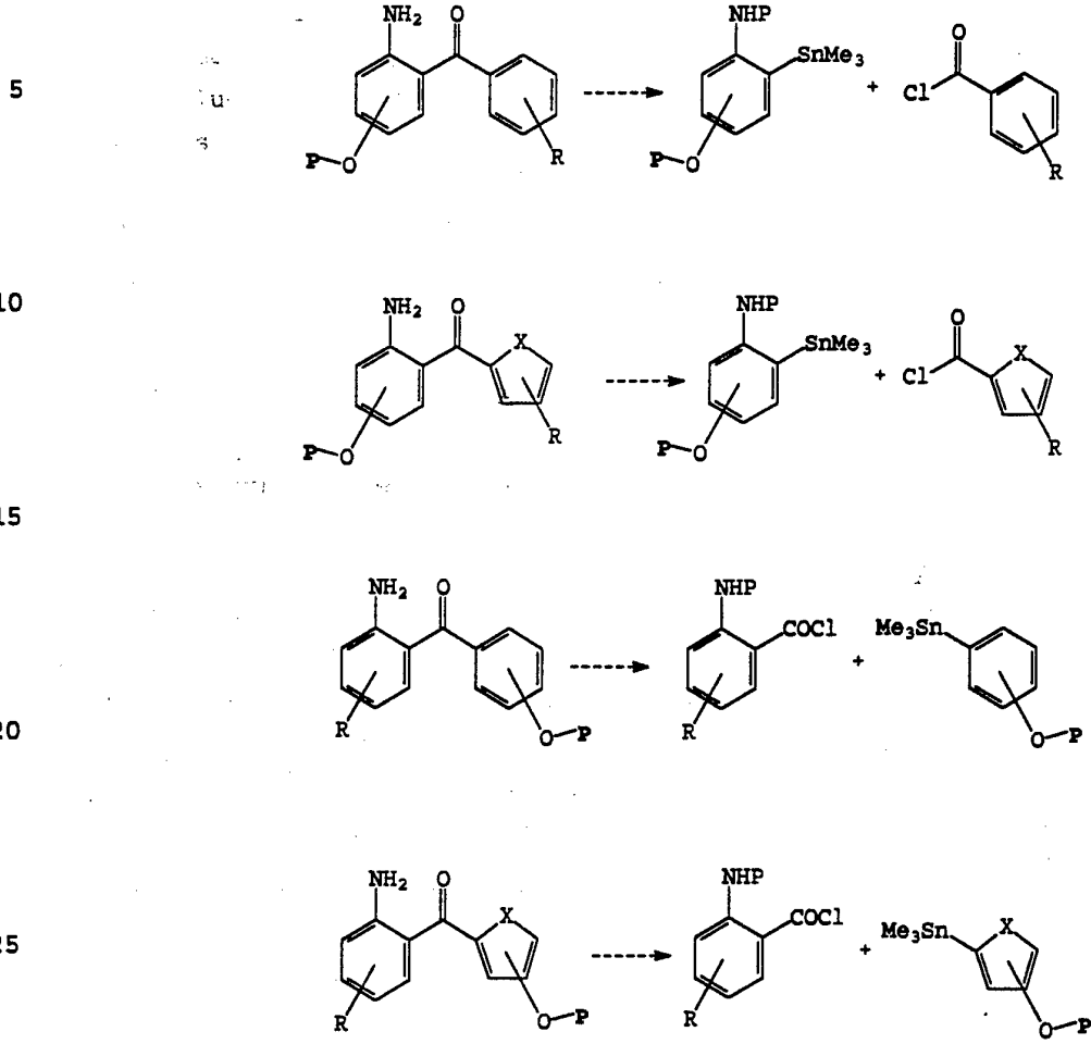
REACTION SCHEME IV
