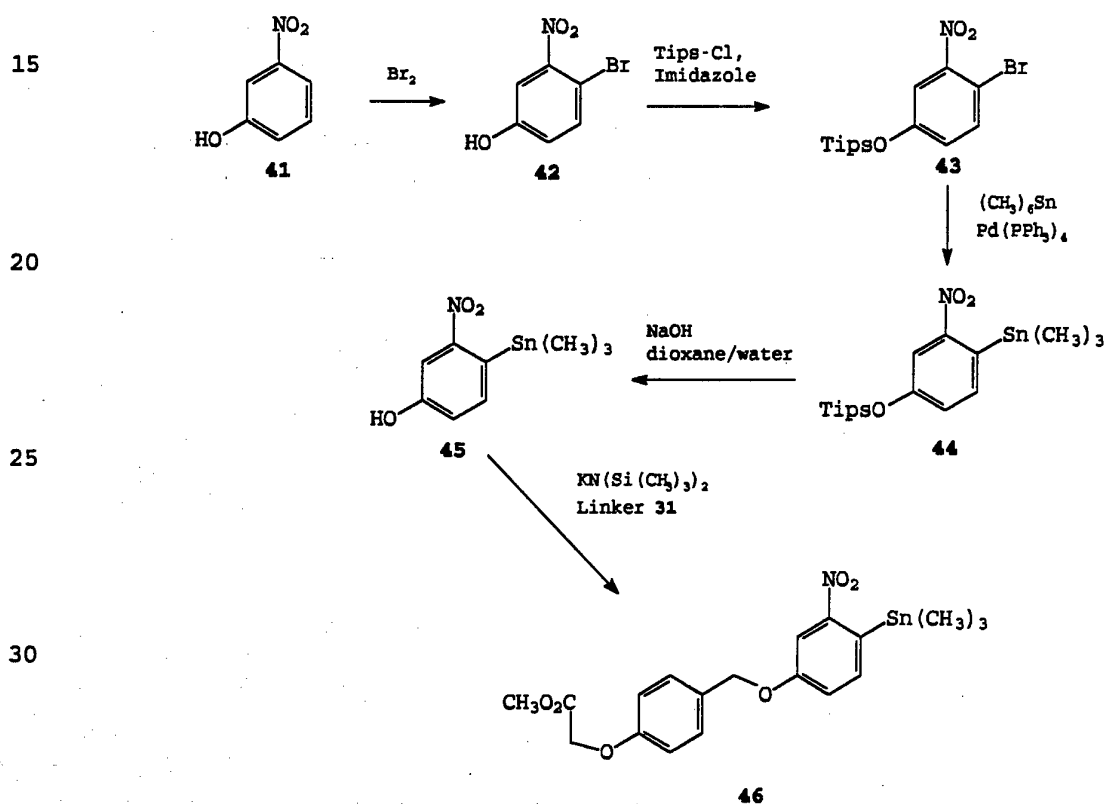
REACTION SCHEME VI
