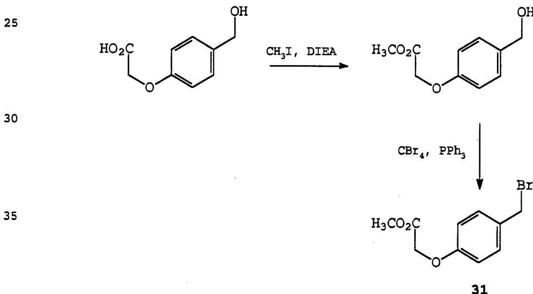
REACTION SCHEME V
