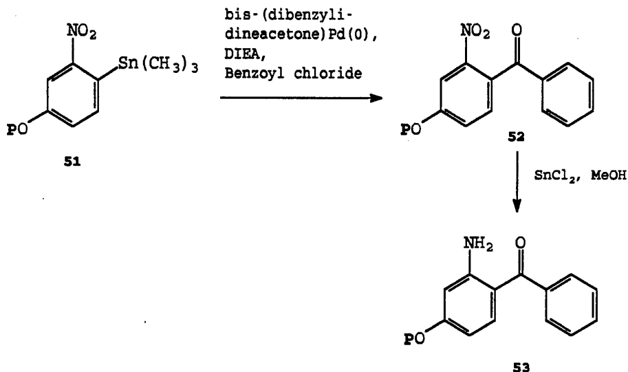
REACTION SCHEME VII
