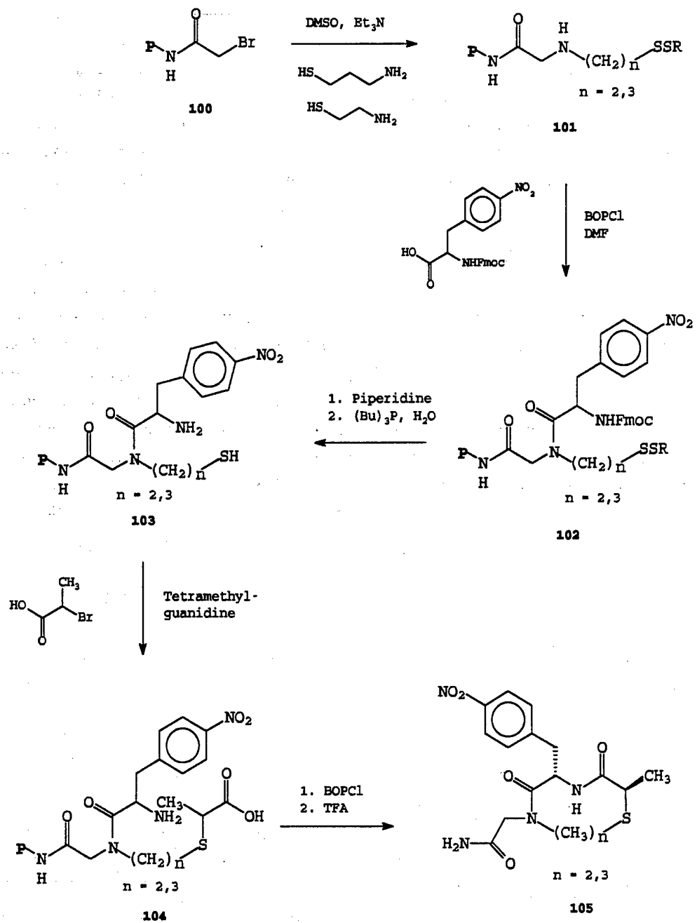
REACTION SCHEME XV
