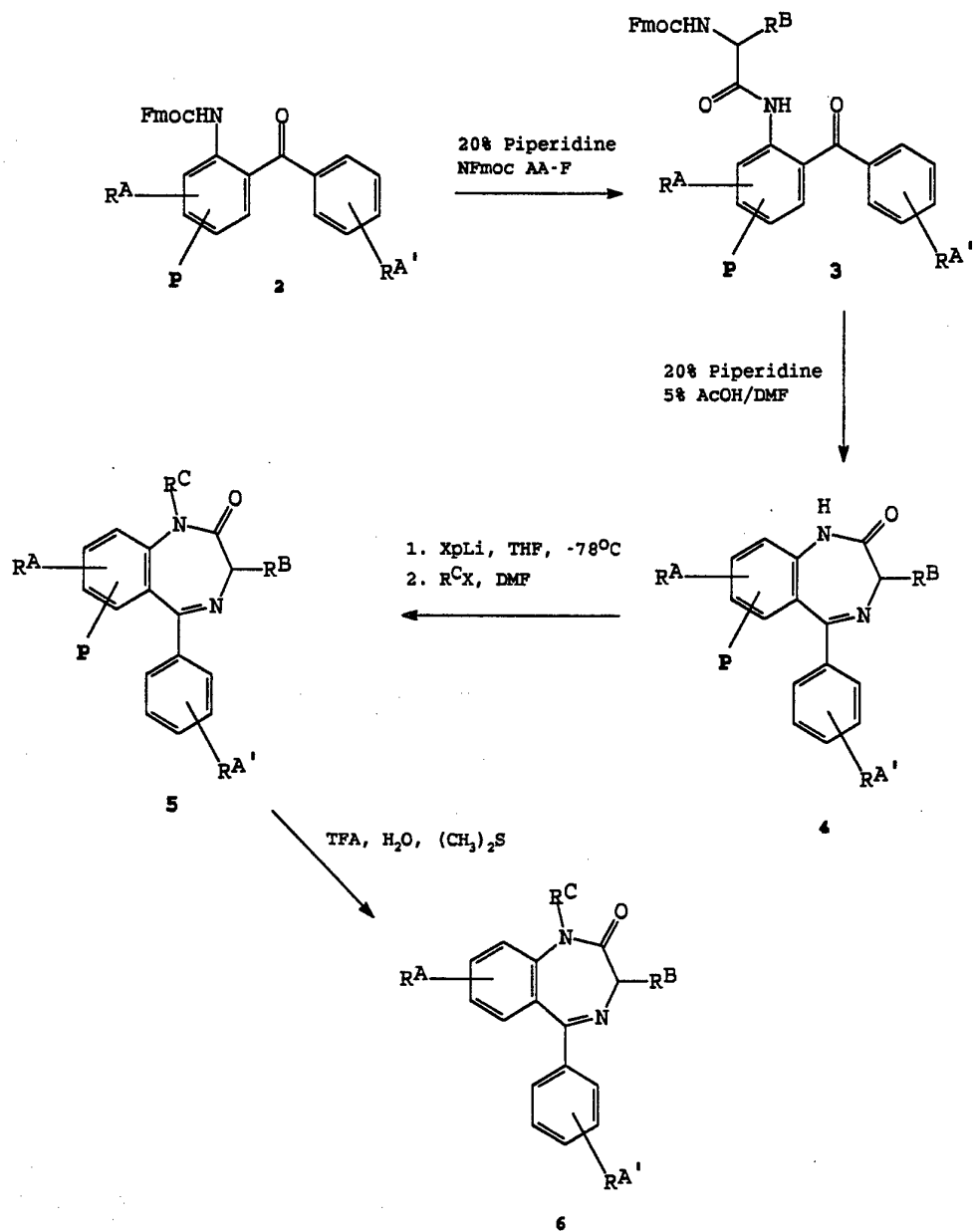
REACTION SCHEME VIII
