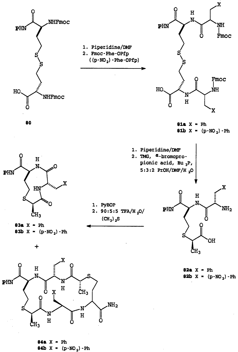
REACTION SCHEME XIII
