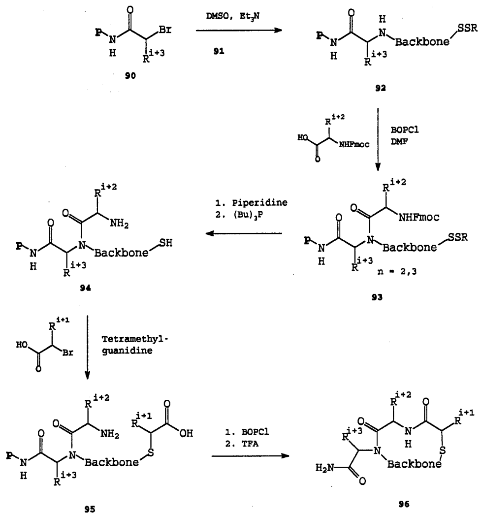
REACTION SCHEME XIV
