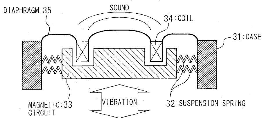
FIG. 10 PRIOR ART
