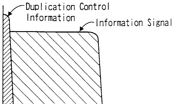
Signal Spectrum After Spectrum De-Spread
