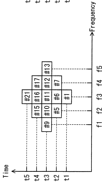
FIG. 77A Modulated signal z1
