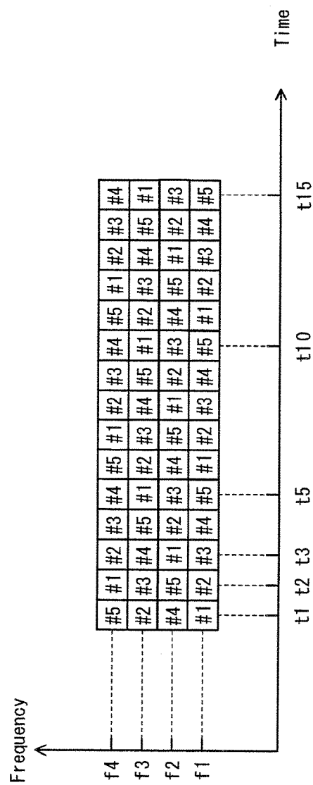
FIG. 65B Modulated A signal z2
