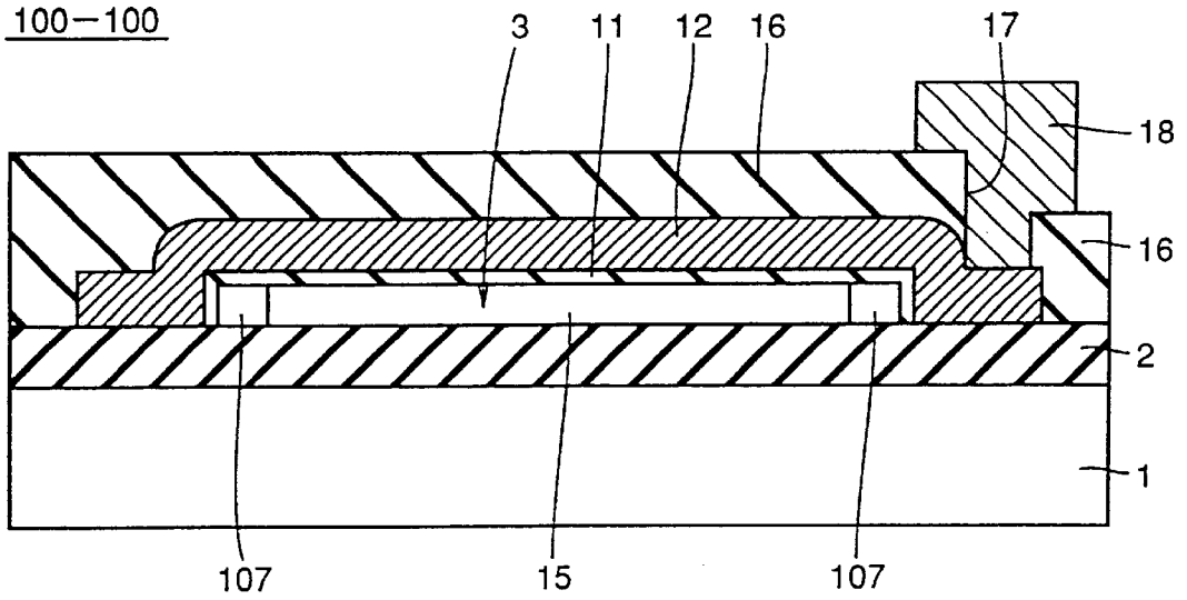
FIG.30 PRIOR ART
