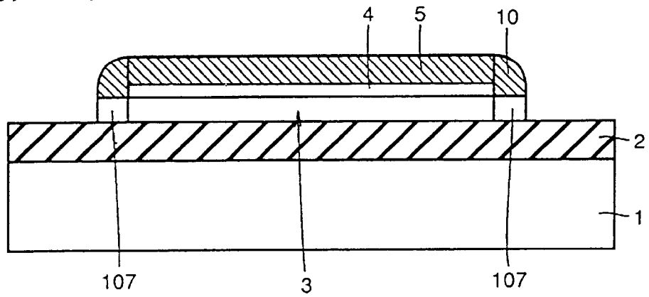
FIG.37 PRIOR ART
