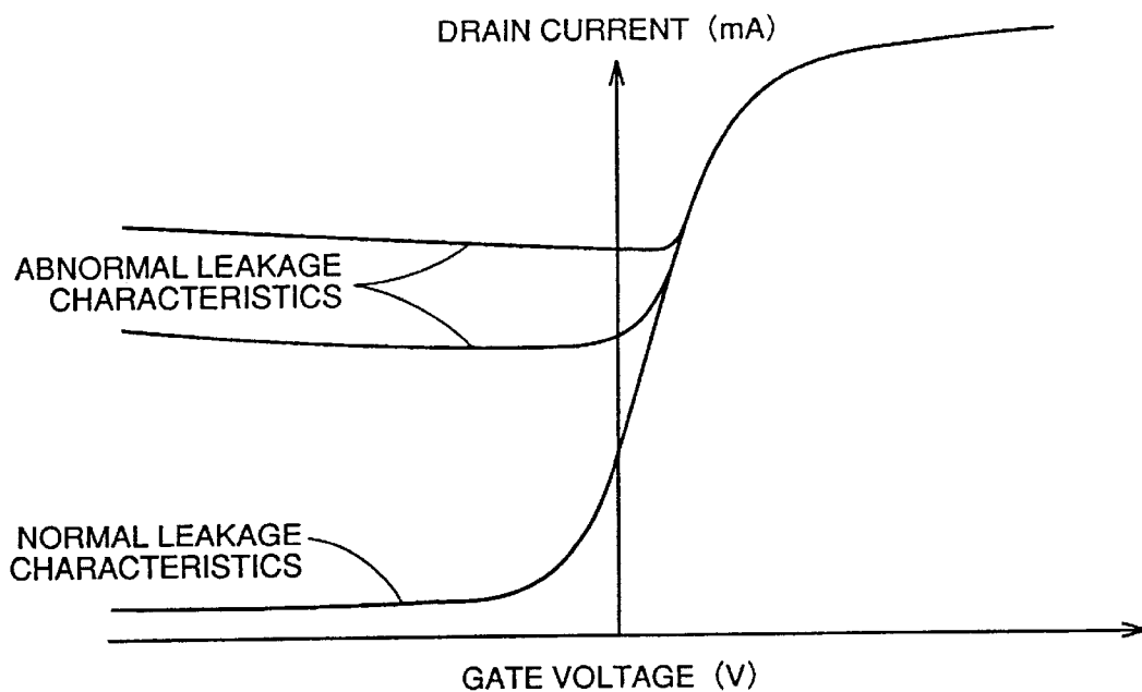
FIG.45 PRIOR ART
