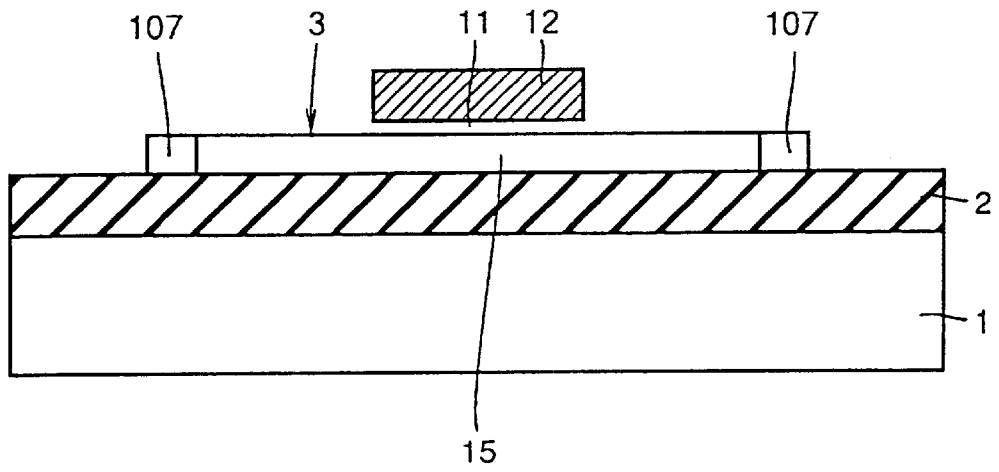
FIG. 40 PRIOR ART
