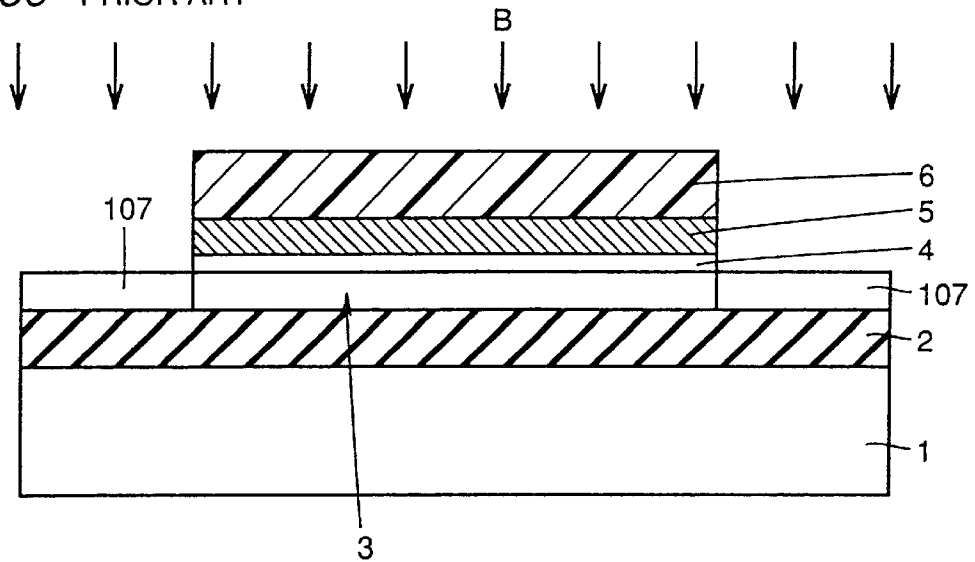
FIG.36 PRIOR ART
