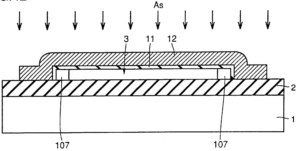
FIG. 42 PRIOR ART
