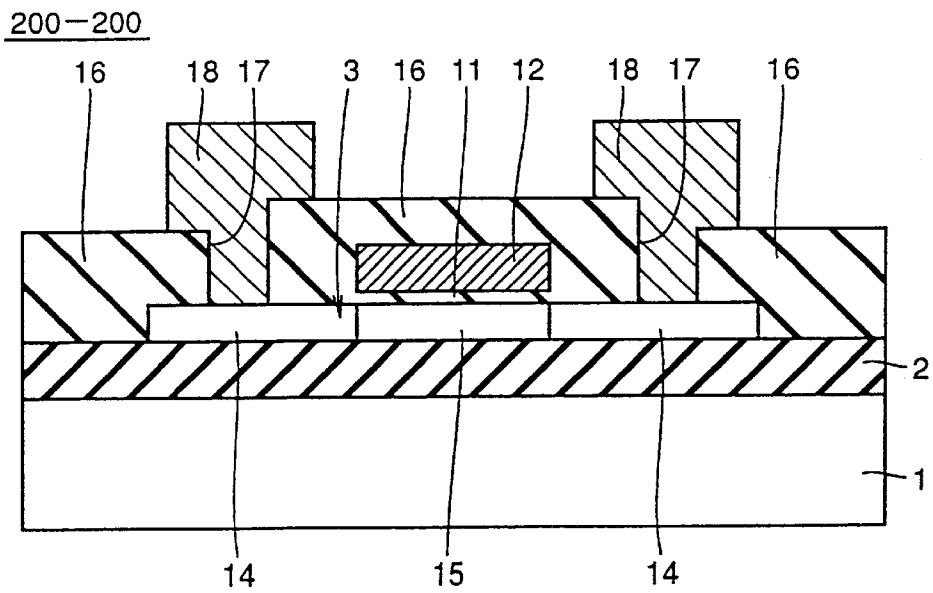
FIG.31 PRIOR ART
