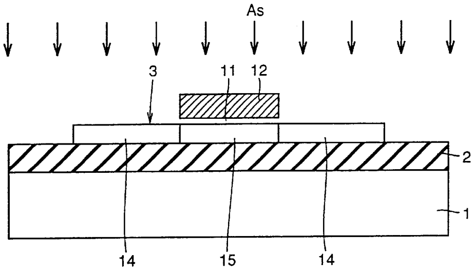
FIG. 43 PRIOR ART
