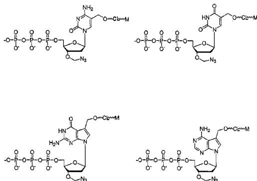
3'-O-azidomethyl nucleotides with cleavable dyes/markers attached via the hydroxymethyl functions on the BASE. CL = cleavable linker.
