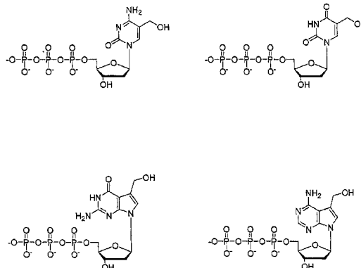
Structures of hydroxymethyl nucleotides after the cleavage of the dyes and the 3'-O- protective groups.
