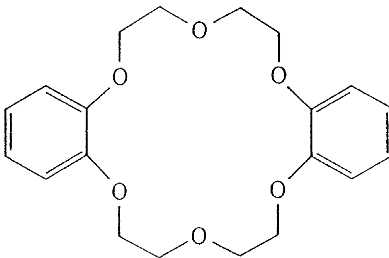
DIBENZOYL-18-CROWN-6
