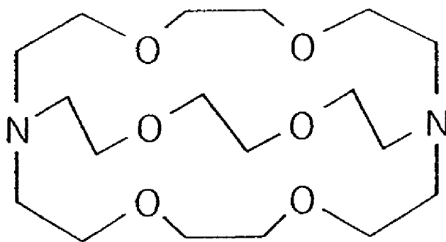
CRYPTAND [2.2.2]
