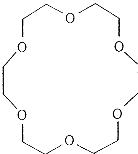
18-CROWN-6
