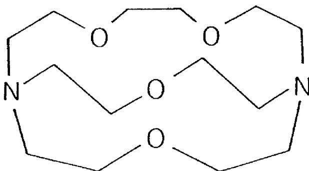
CRYPTAND [2.1.1]
