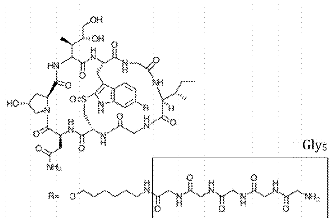
Gly 5 -modified alpha-amanitin
