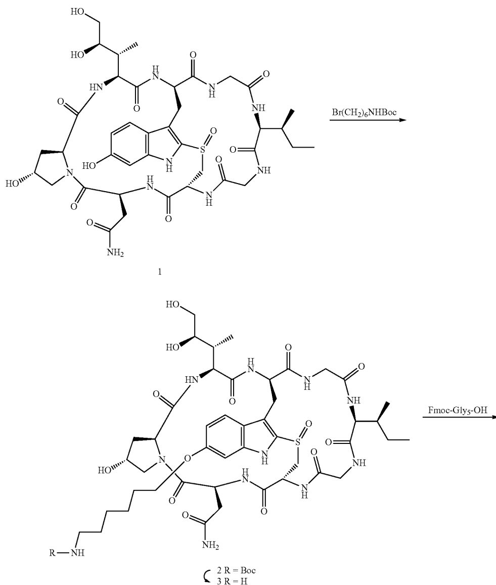
Scheme 1: Synthesis of glycine-modified alpha-amanitin
