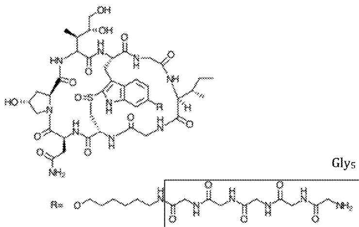
Gly 5 -alpha-amanitin (III)
