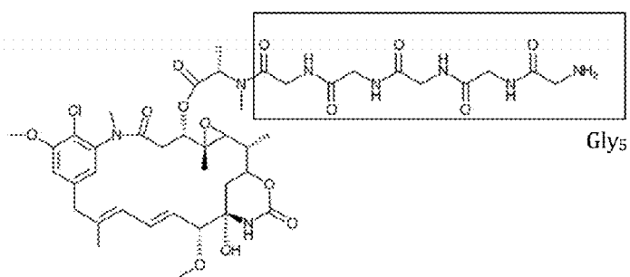
Gly 5 -modified maytansine
