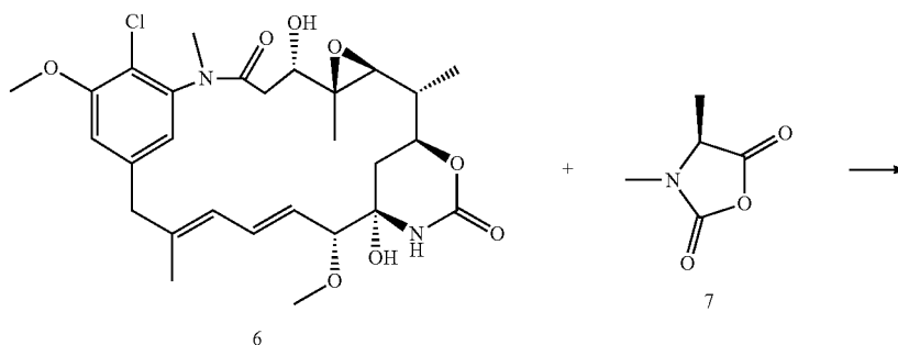
Scheme 2: Synthesis of glycine-modified maytansine
