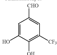
3,4-Dihydroxy-5-(trifluoromethyl)benzaldehyde
