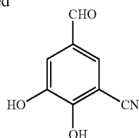
5-Formyl-2,3-dihydroxybenzonitrile
