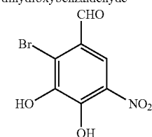
2-Bromo-3,4-dihydroxy-5-nitrobenzaldehyde
