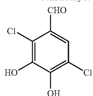
2,5-Dichloro-3,4-dihydroxybenzaldehyde
