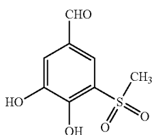
3,4-Dihydroxy-5-(methylsulfonyl)benzaldehyde
