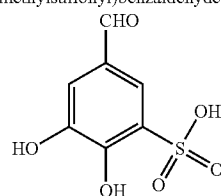
5-formyl-2,3-dihydroxybenzenesulfonic acid
