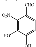
3,4-Dihydroxy-2-nitrobenzaldehyde
