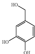
3,4-Dihydroxybenzyl alcohol (DHBA)
