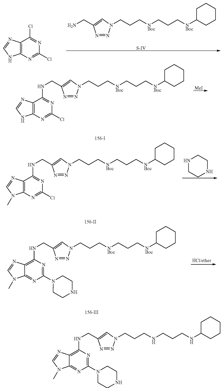
Compound 156
