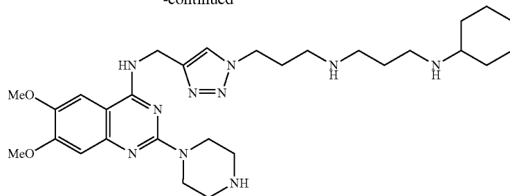
compound 157
