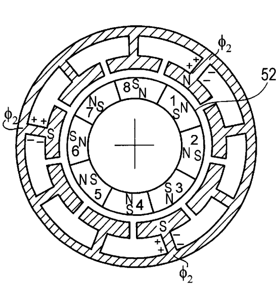
Fig. 8C (Prior Art)
