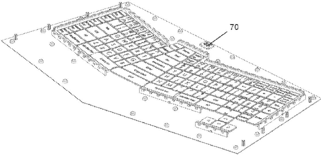
FIG. 12 – Integral Receptacle
