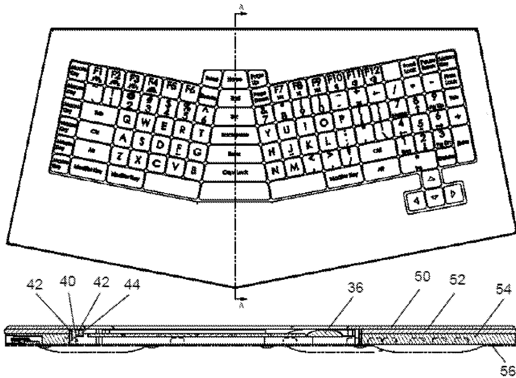
FIG. 6 – Crossed-sectional View of Present Invention
