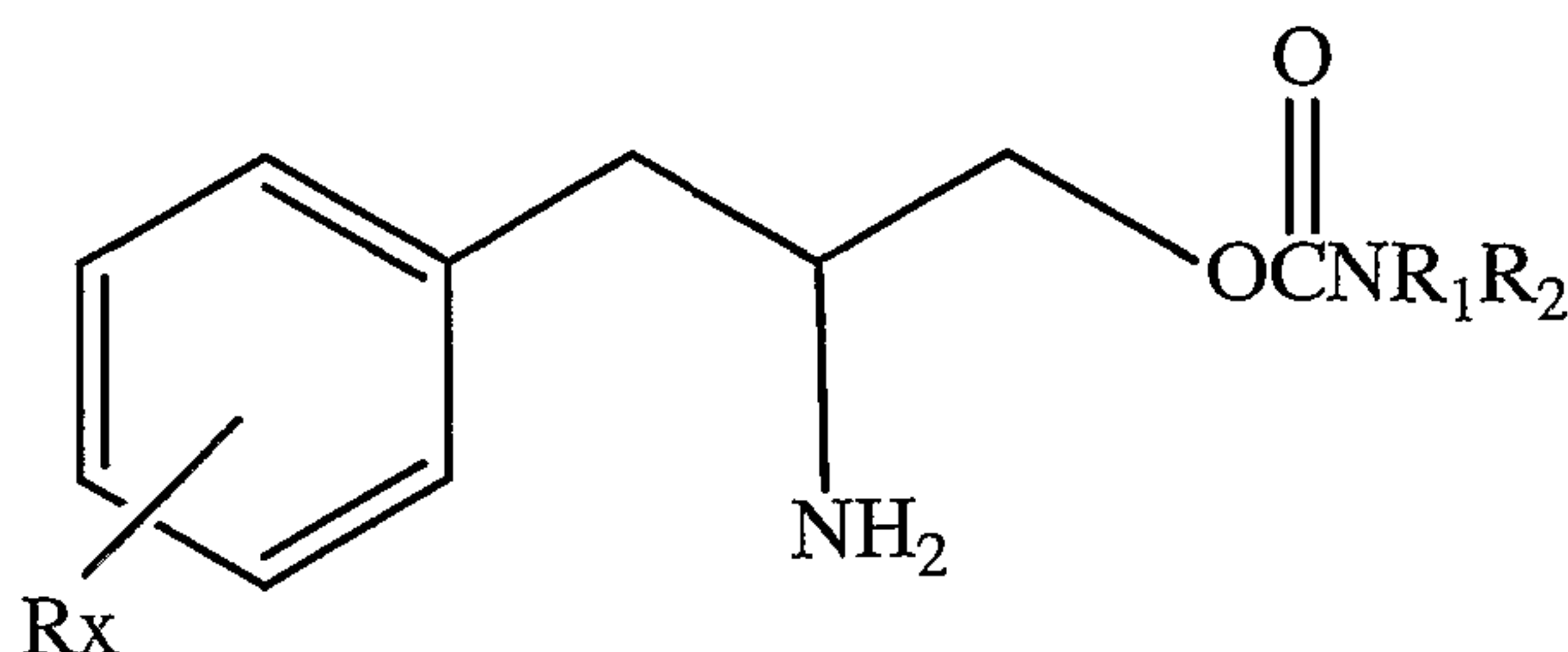
(I)
