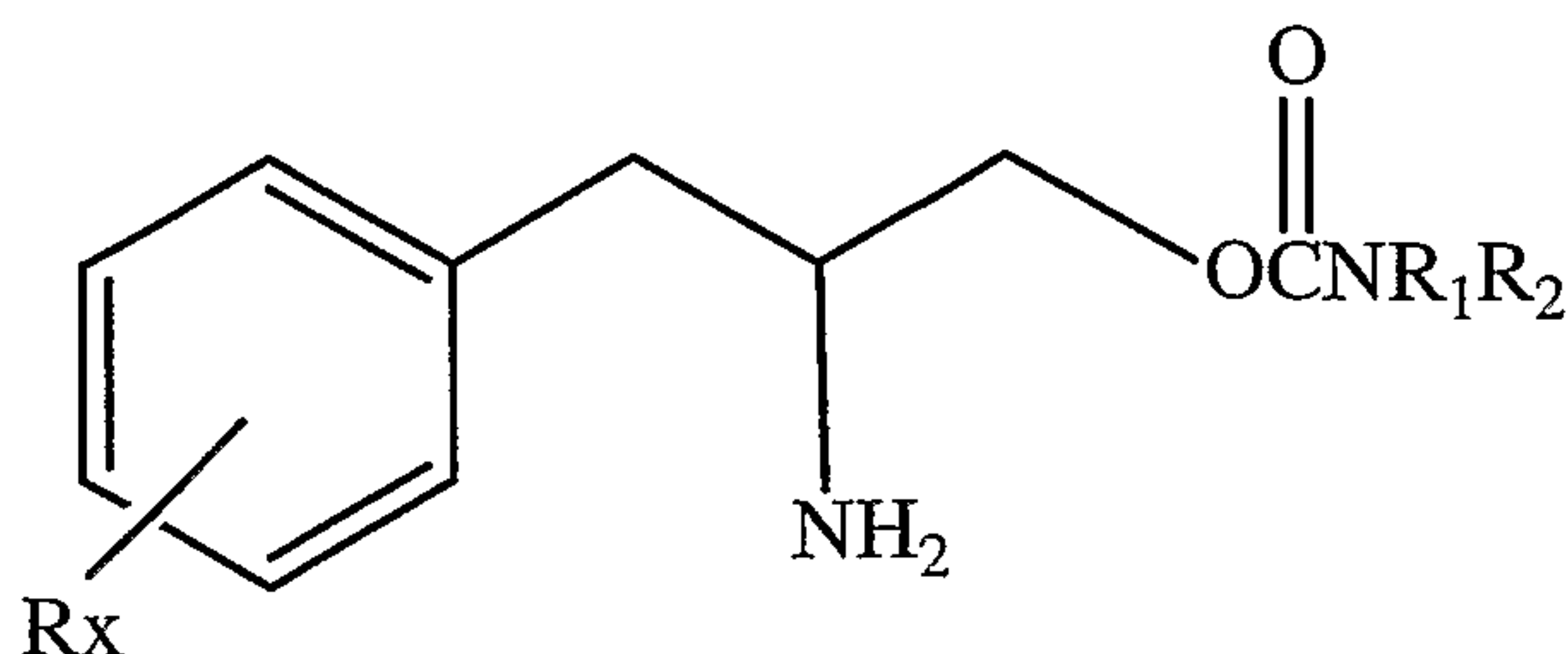
(I)
