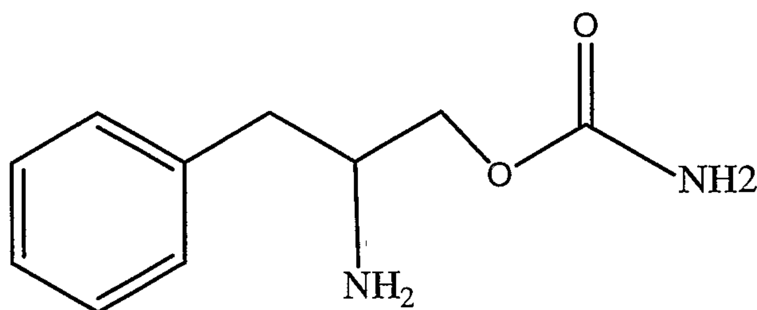
. Formula Ib
