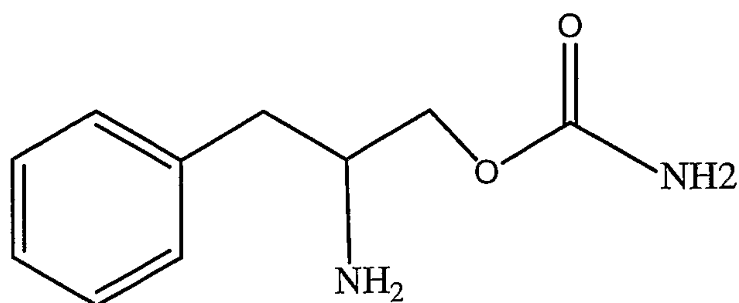
. Formula Ia
