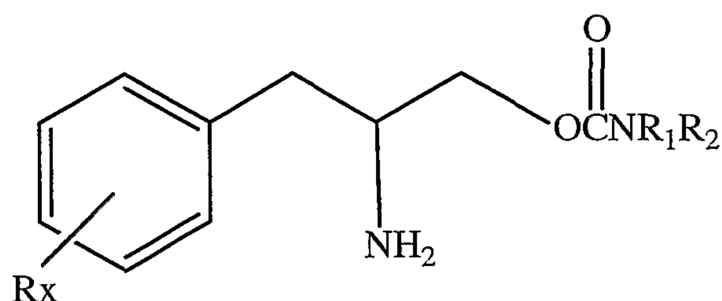
(I)
