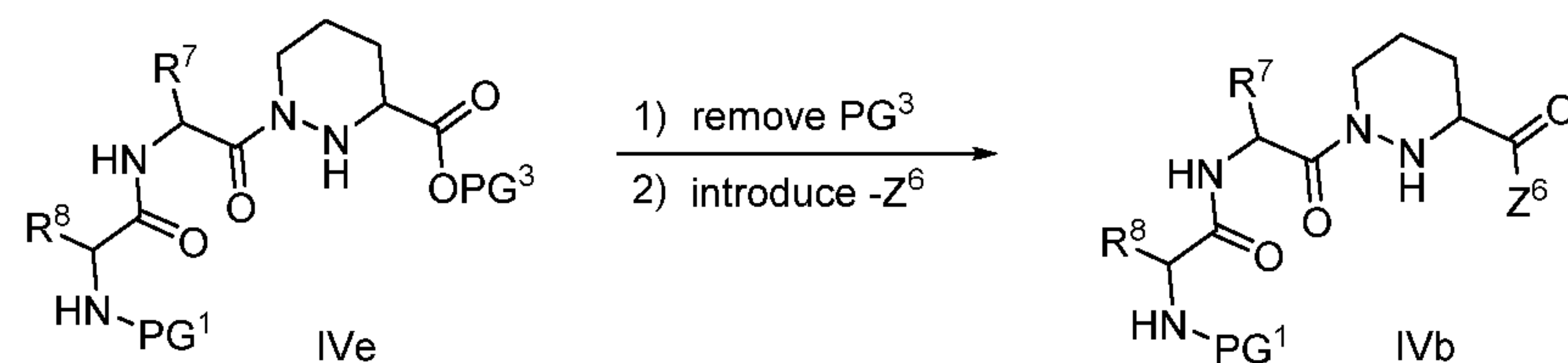
Scheme 4
