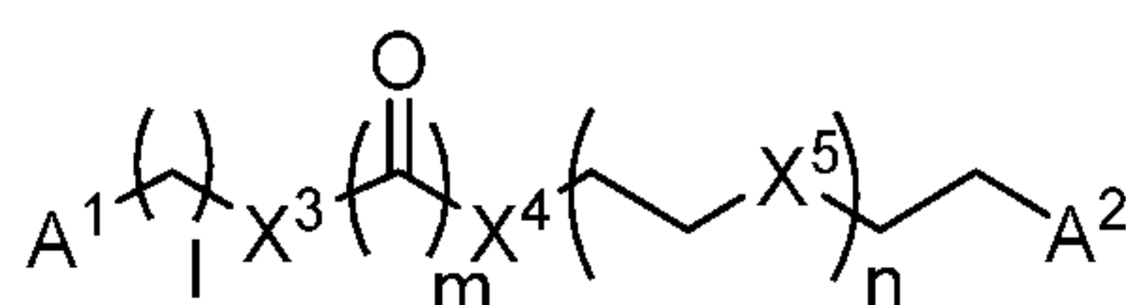
Formula VI
