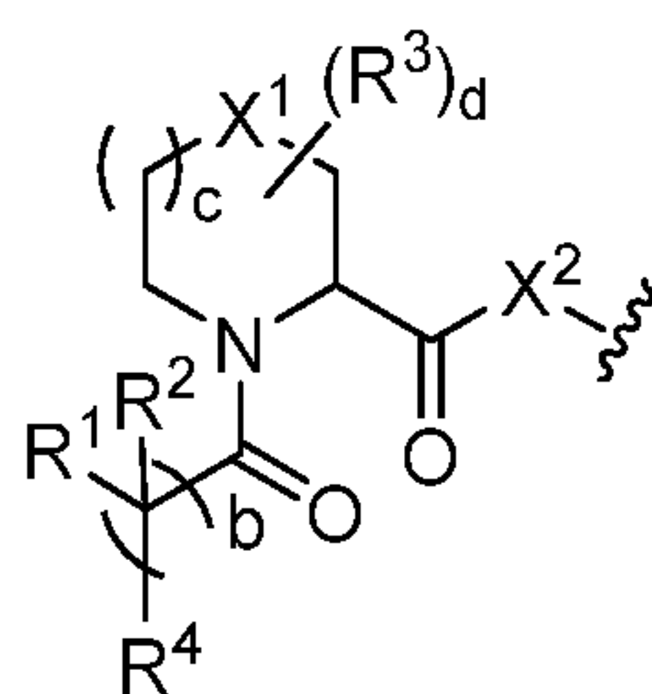
Formula VIIa
