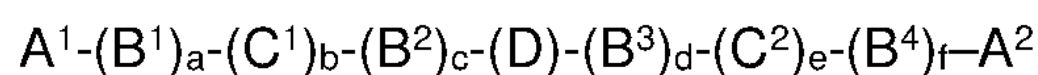
Formula XIX
