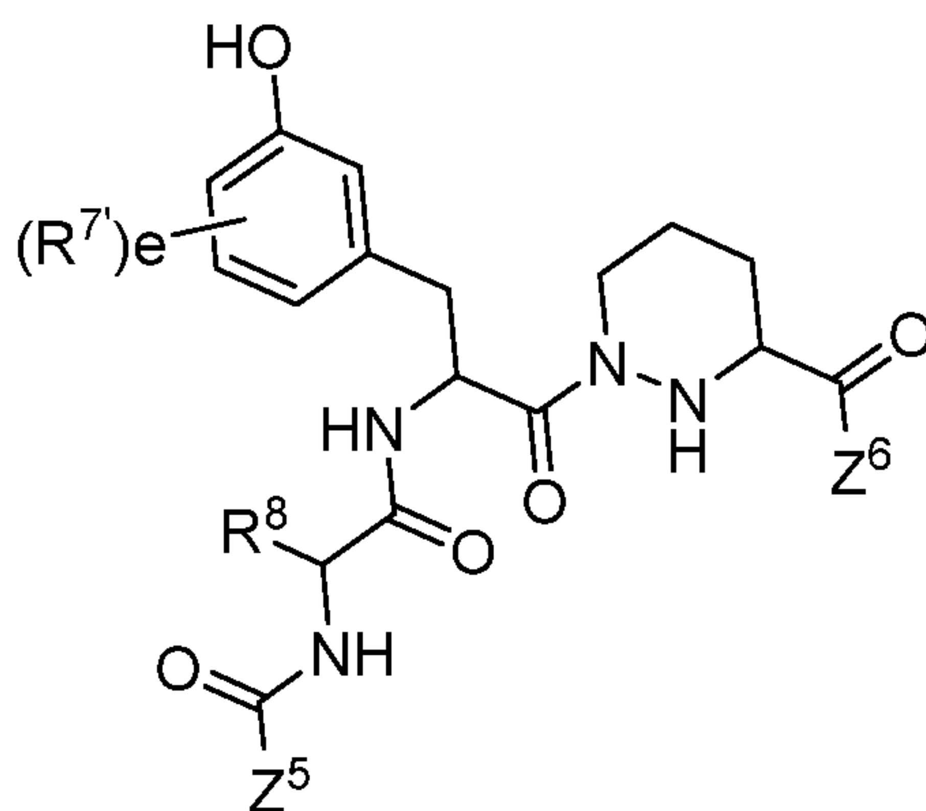
Formula IVa
