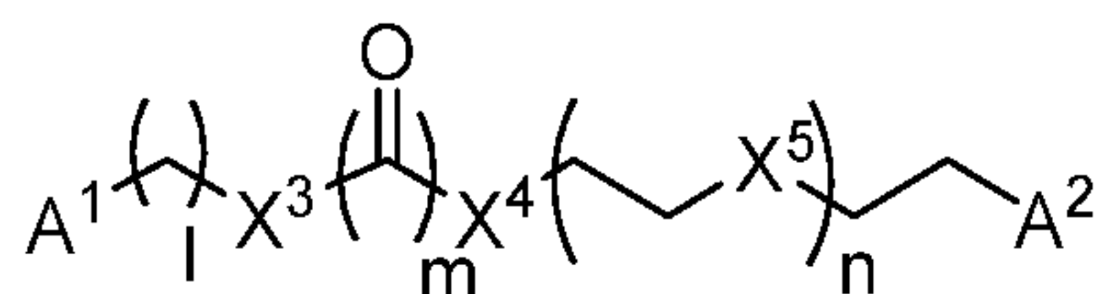
Formula VI
