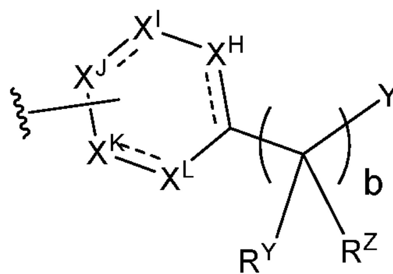
Formula Ip
