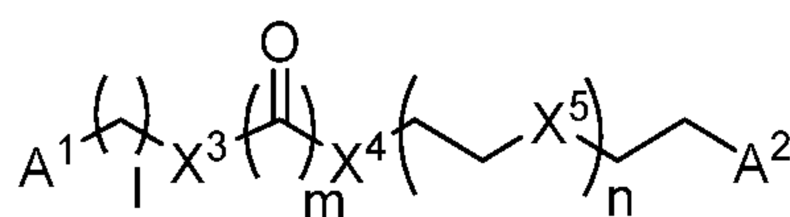
Formula VI
