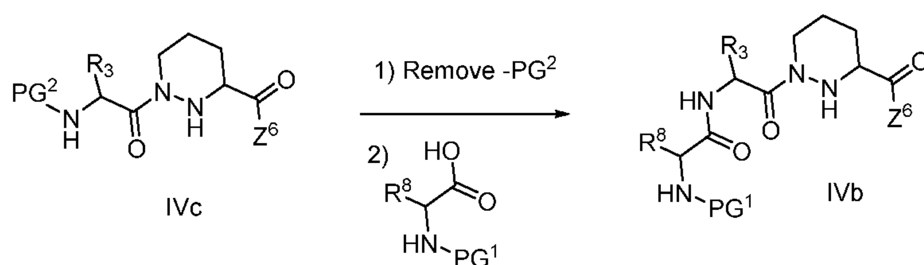
Scheme 2
