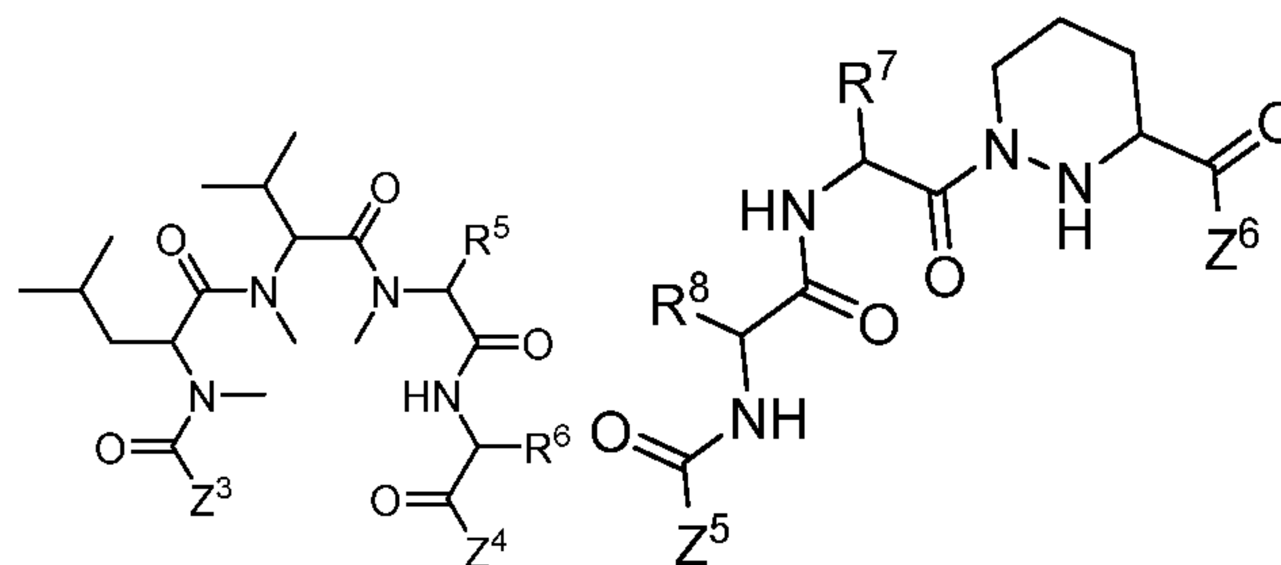
Formula III
