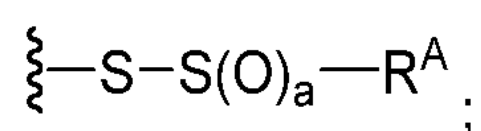
Formula Ia
