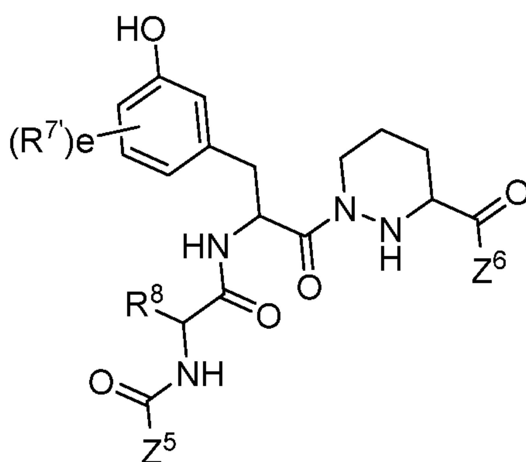
Formula IVa
