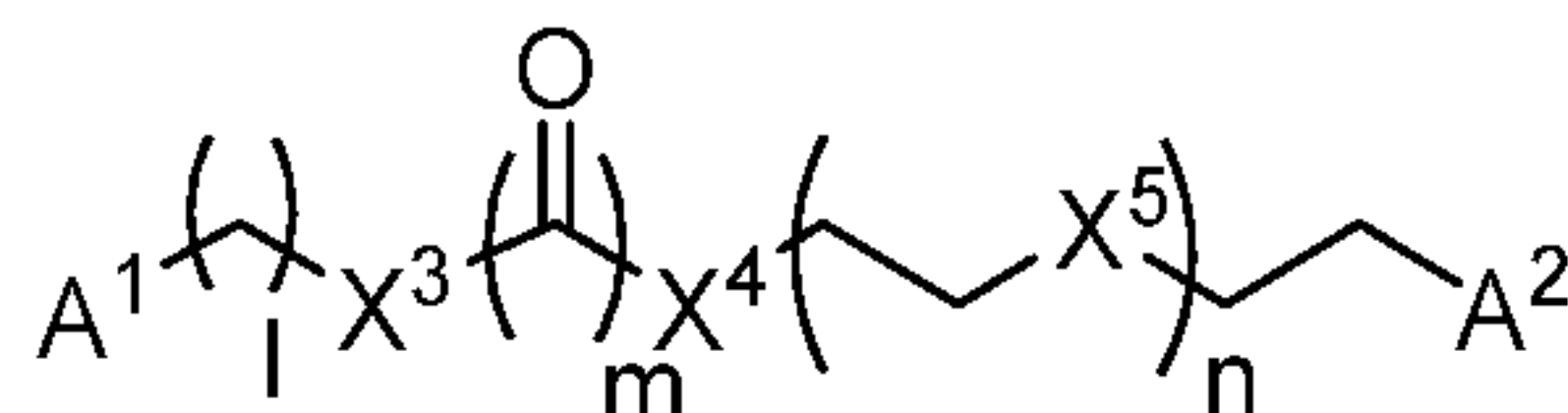
Formula VI
