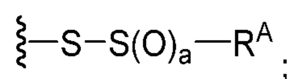
Formula I
