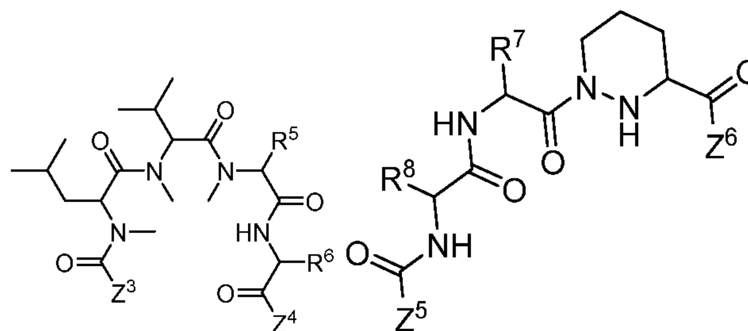
Formula III
