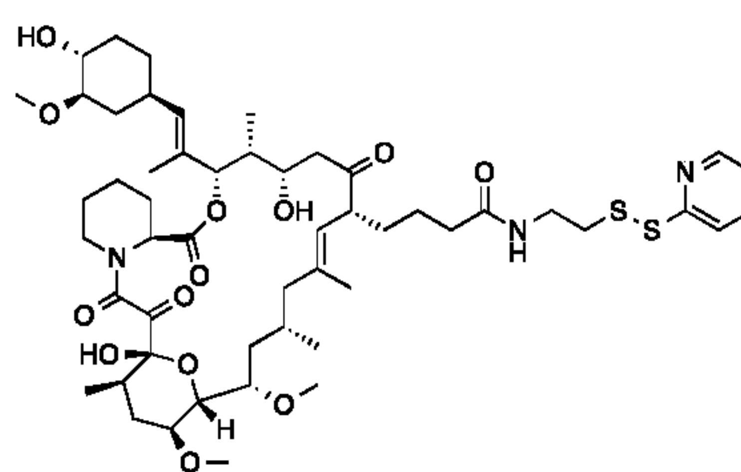
C2-FK506
