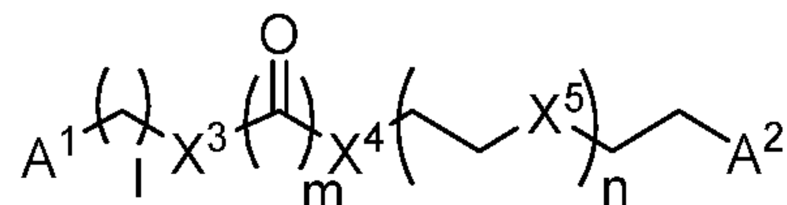
Formula VI
