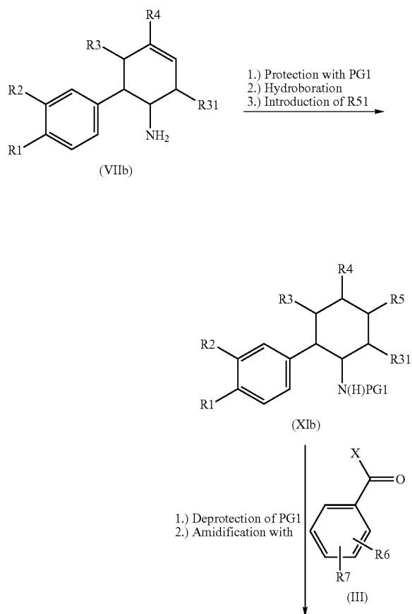
Reaction scheme 6:
