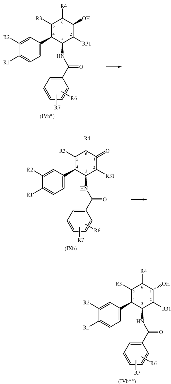
Reaction scheme 4:
