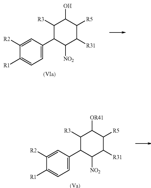
Reaction scheme 1:
