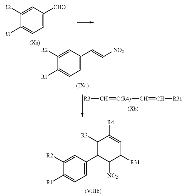
Reaction scheme 5:
