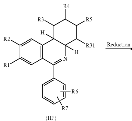
Reaction scheme 1':
