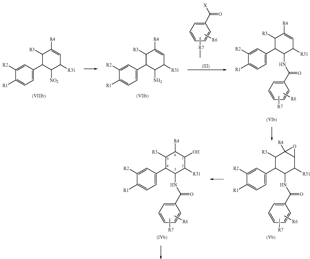
Reaction scheme 3:
