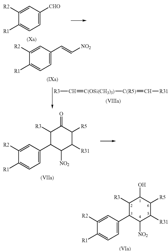
Reaction scheme 2:
