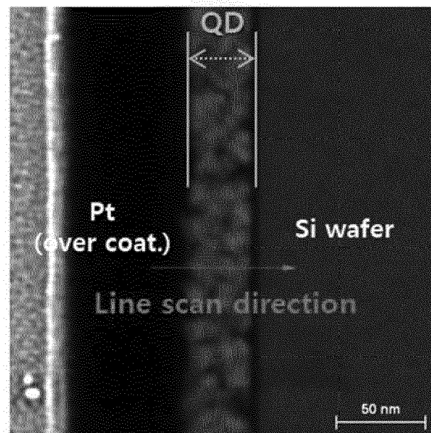
Cl distribution
