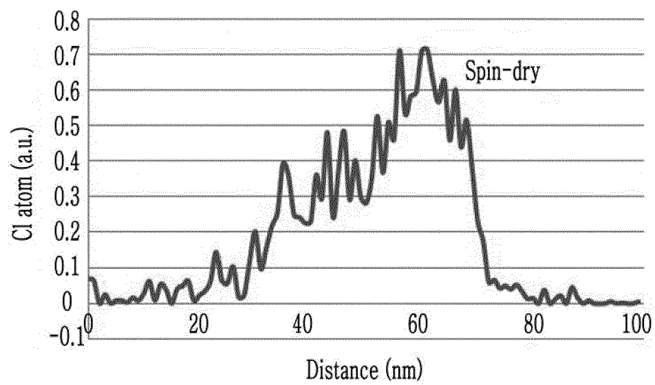
Cl distribution
