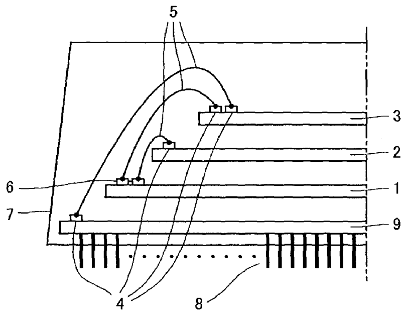
SIP STRUCTURE AFTER INSERTION OF TRACE CHIP
