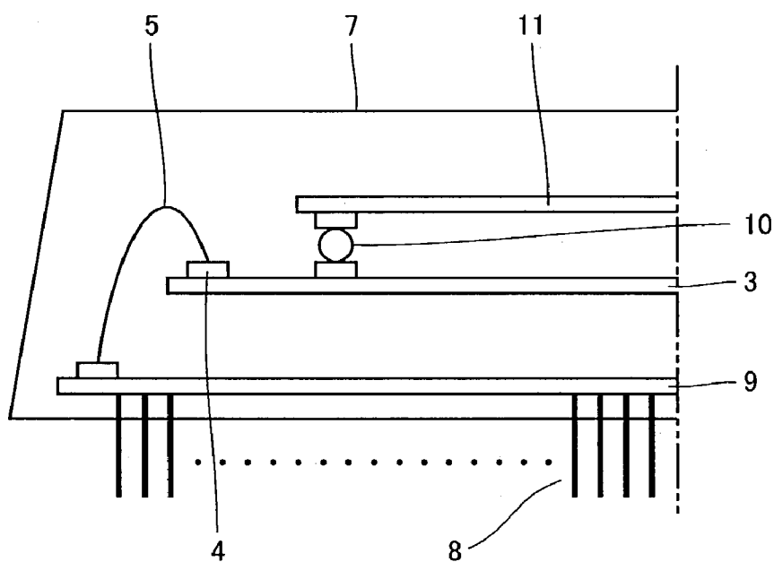
SIP STRUCTURE BEFORE INSERTION OF TRACE CHIP
