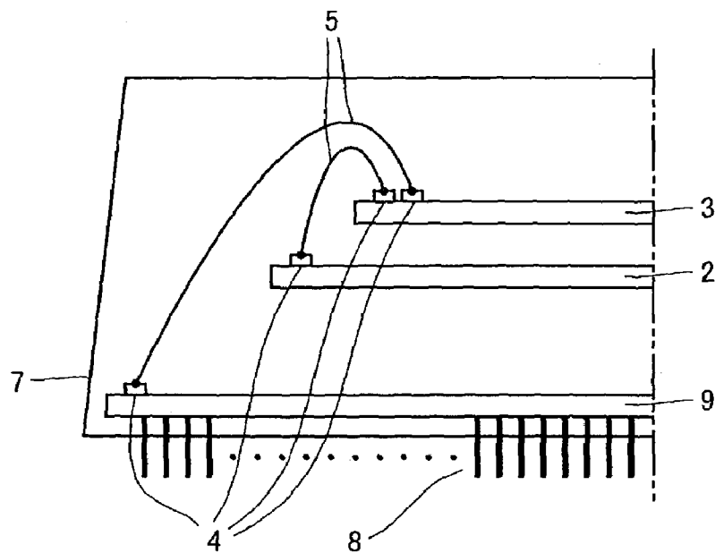
SIP STRUCTURE BEFORE INSERTION OF TRACE CHIP
