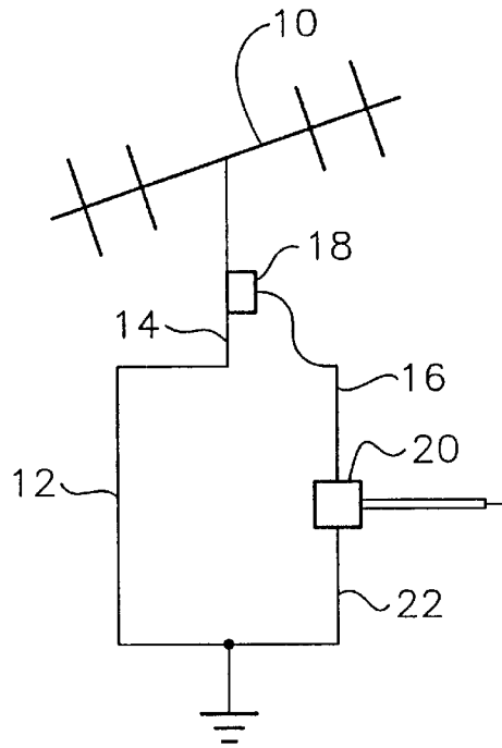
Fig. 1 Prior Art
