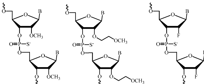
2'-O-Methyl PS
