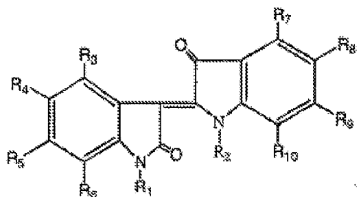
FORMULA (III)
