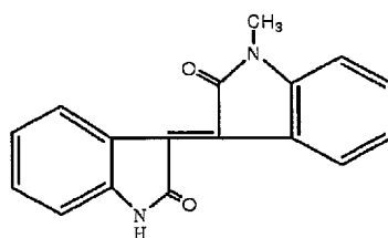
FORMULA (IV)
