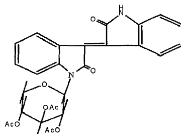
FORMULA (VI).
