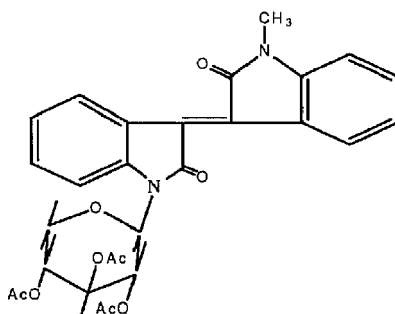
FORMULA (V)
