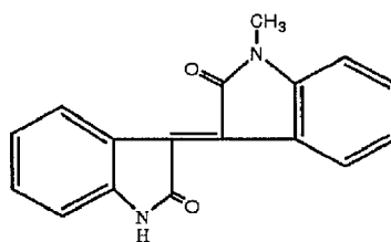
FORMULA (IV)
