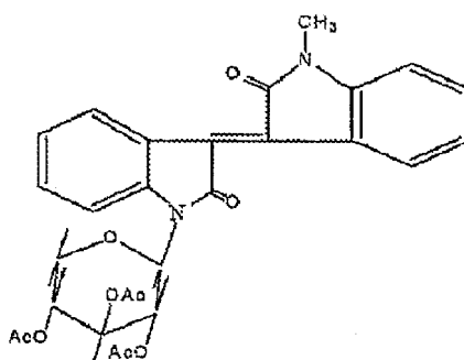
FORMULA (V)
