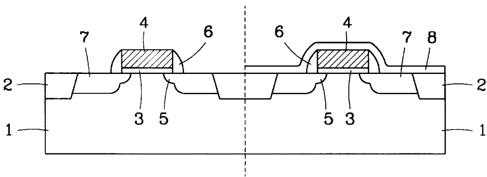
FIG. 1C CONVENTIONAL ART
