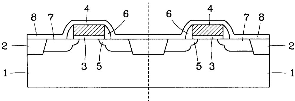
FIG. 1B CONVENTIONAL ART
