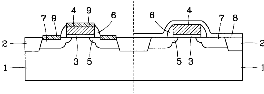
FIG. 1D CONVENTIONAL ART
