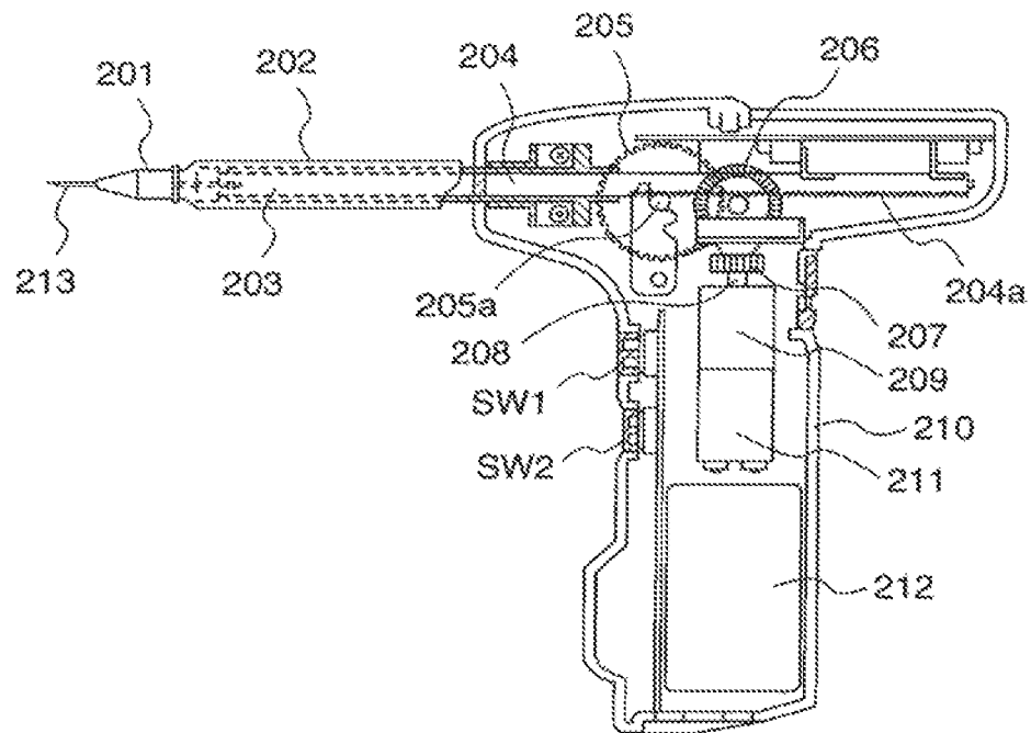
Fig.24 Prior Art
