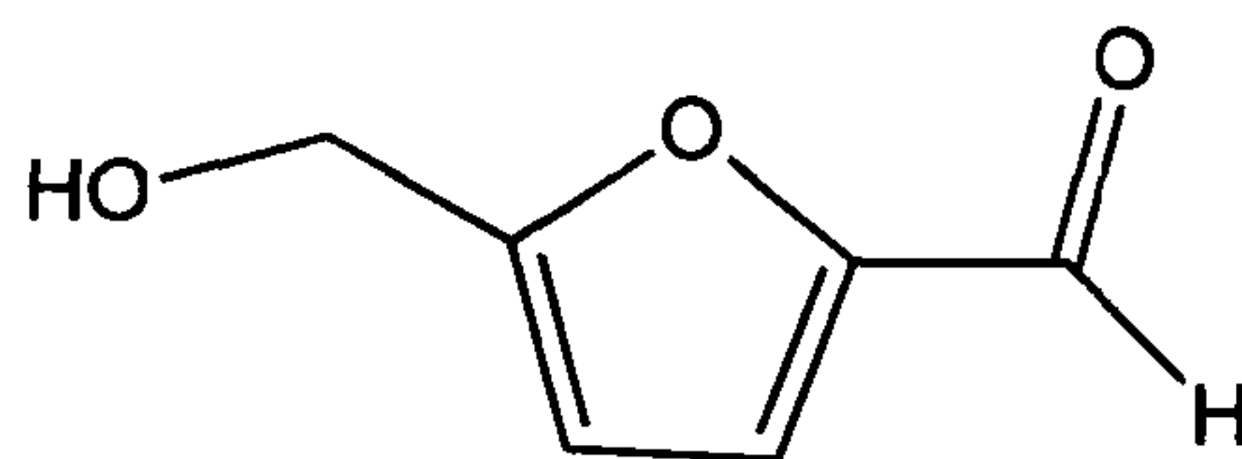
Hydroxymethylfurfural
