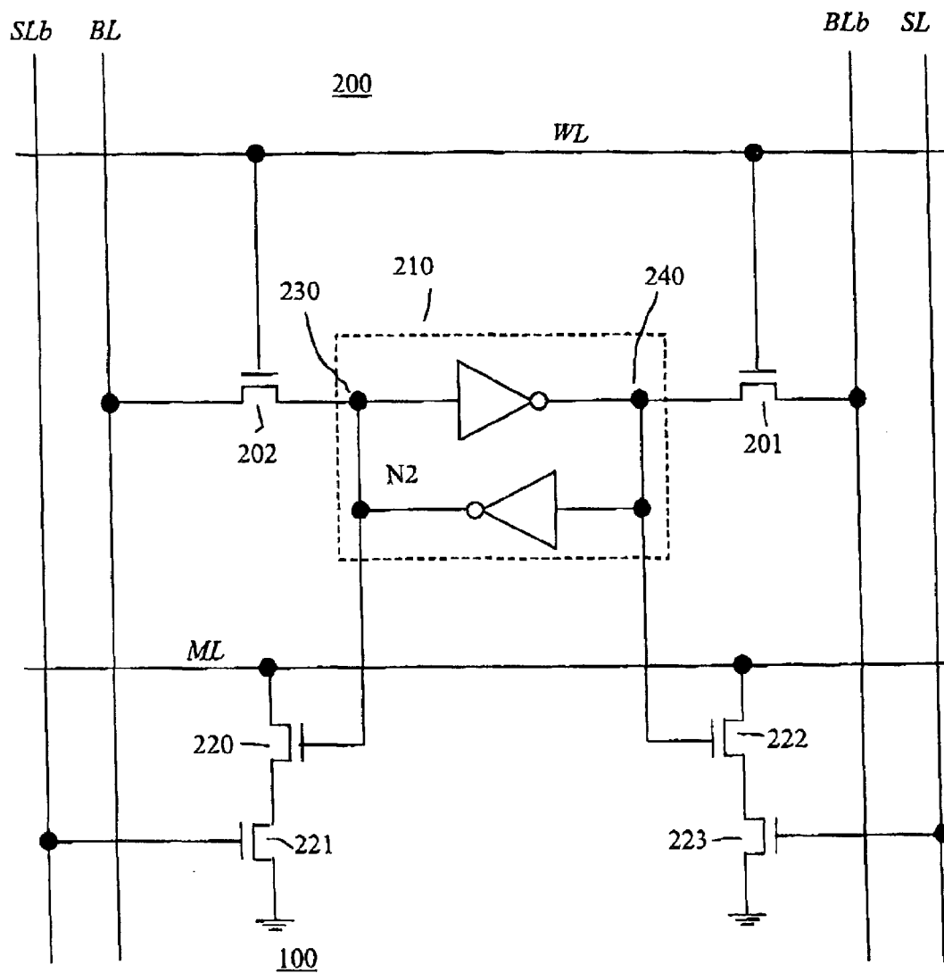
Figure 2 (prior art)
