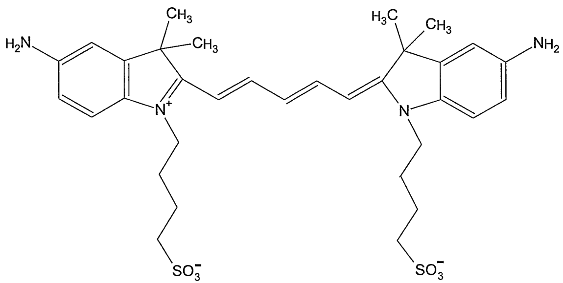
Compound IVa
