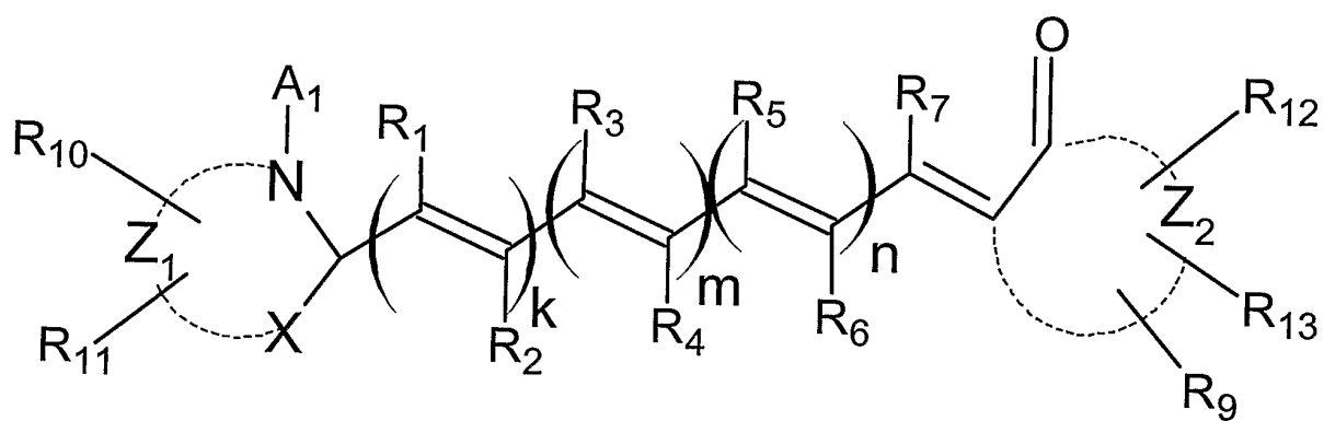
Merocyanine
