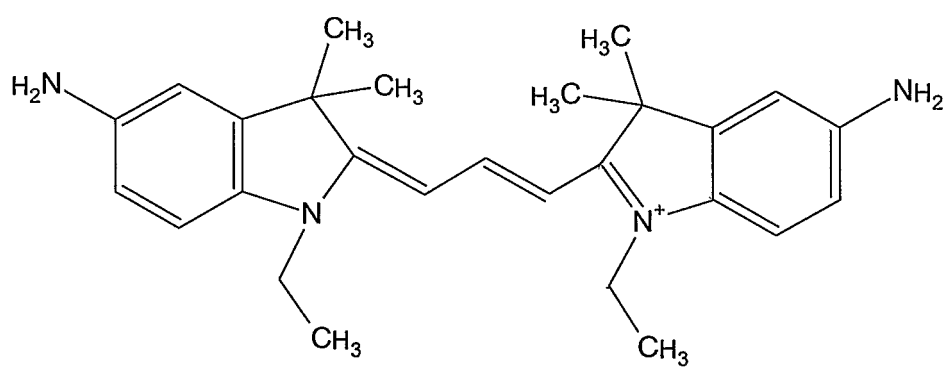
Compound IIIb
