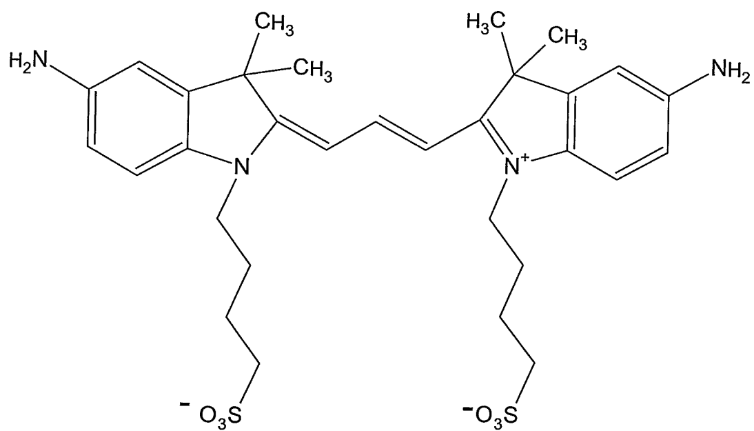
Compound IIIa
