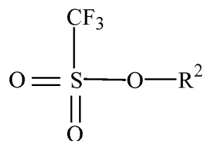
Formula (IIA)
