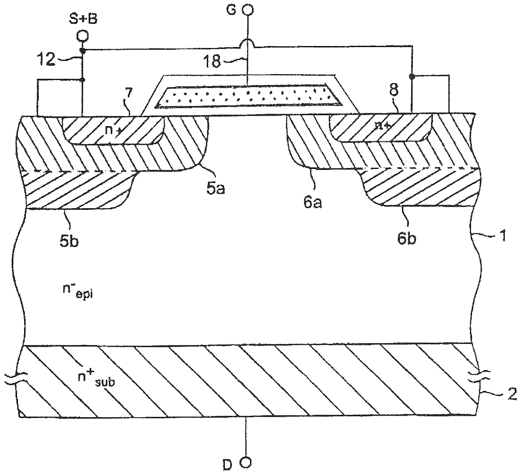
CONVENTIONAL MOSFET
