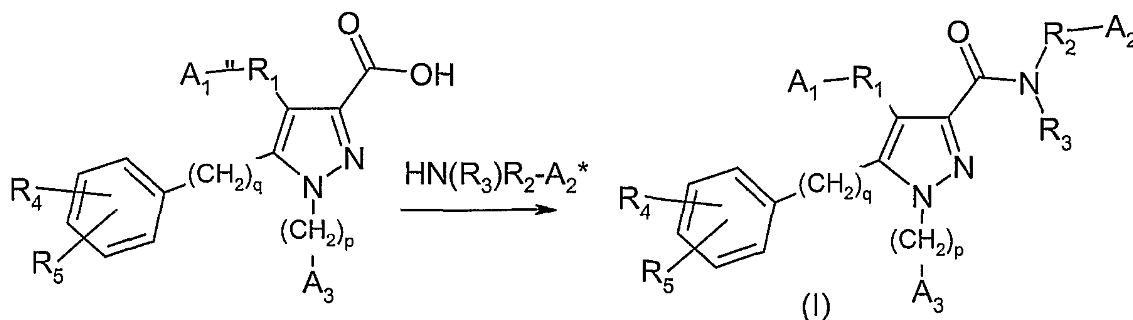
Scheme 1
