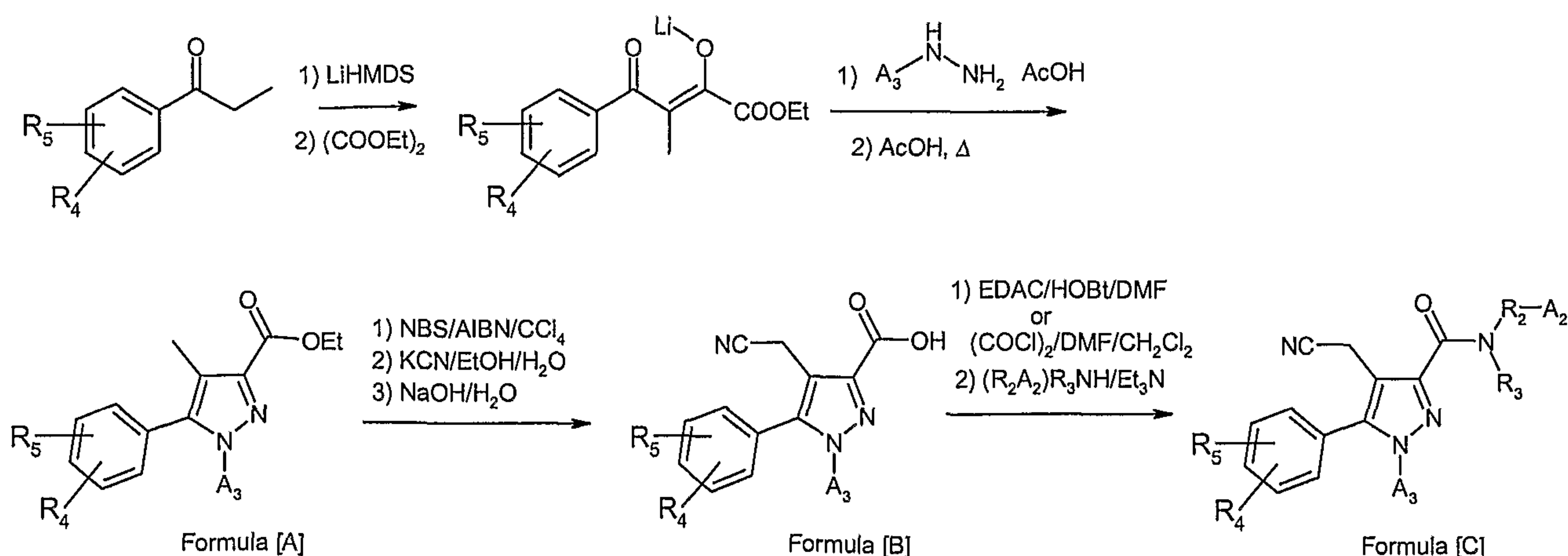
Scheme 6
