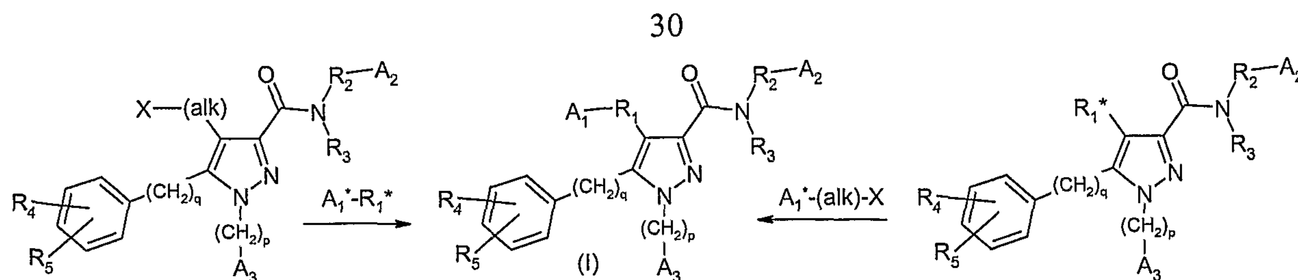
Scheme 3
