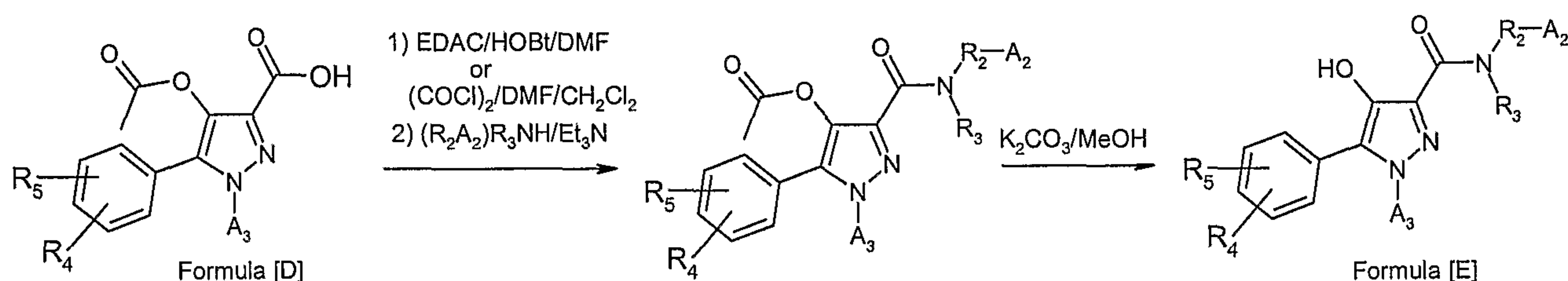
Scheme 7
