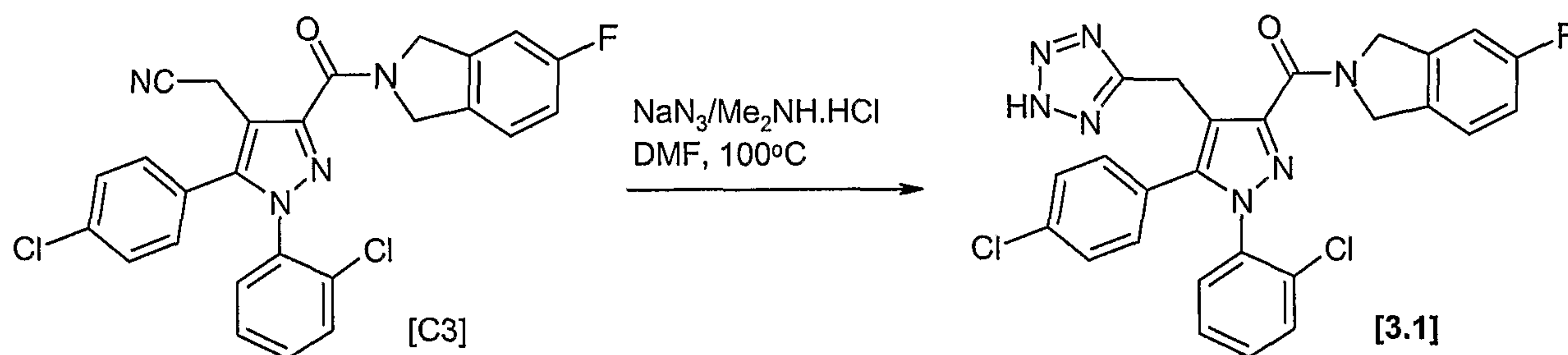
Scheme 10
