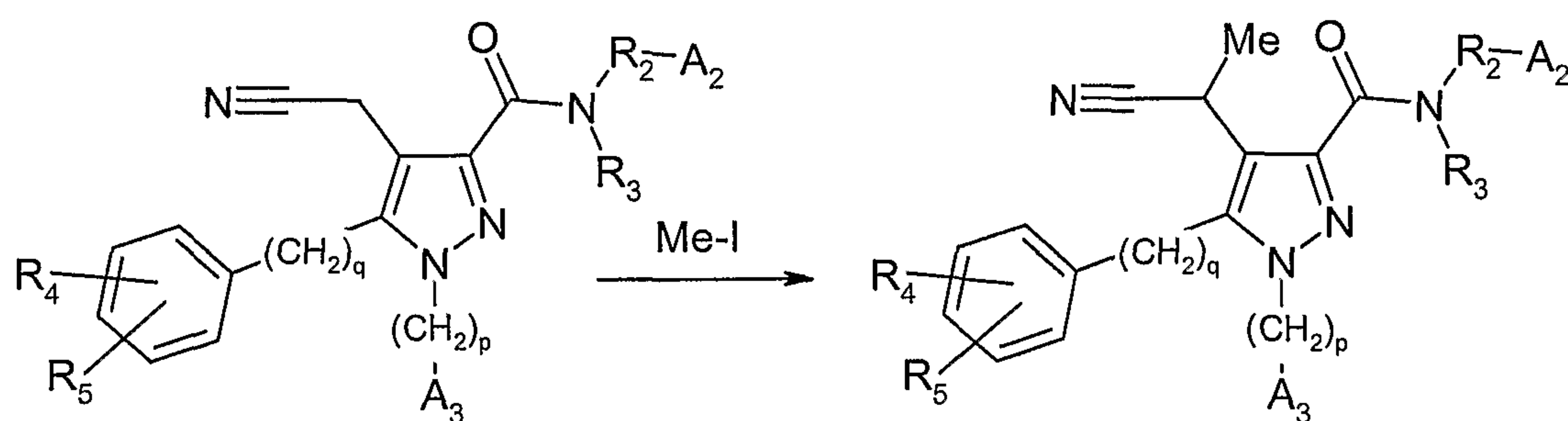
Scheme 4
