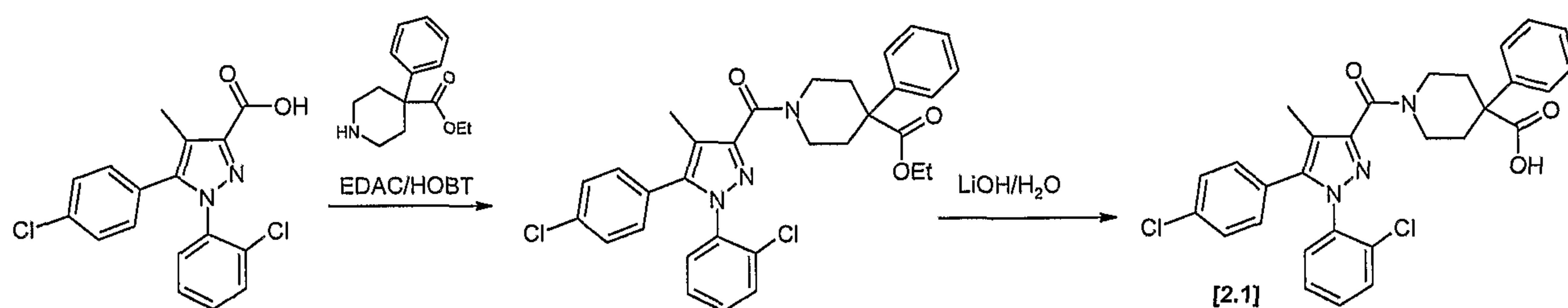
Scheme 9
