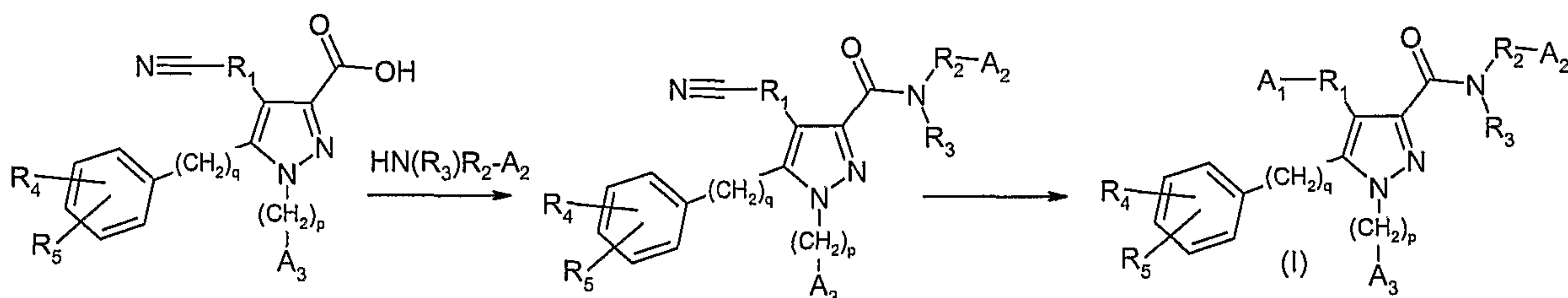
Scheme 2
