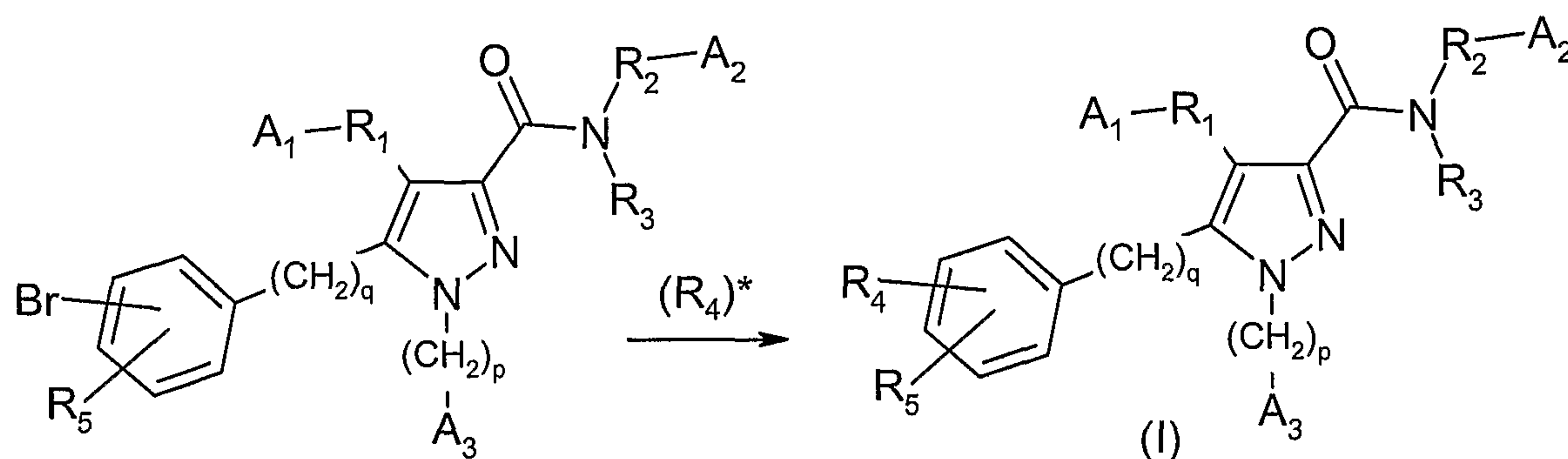
Scheme 5
