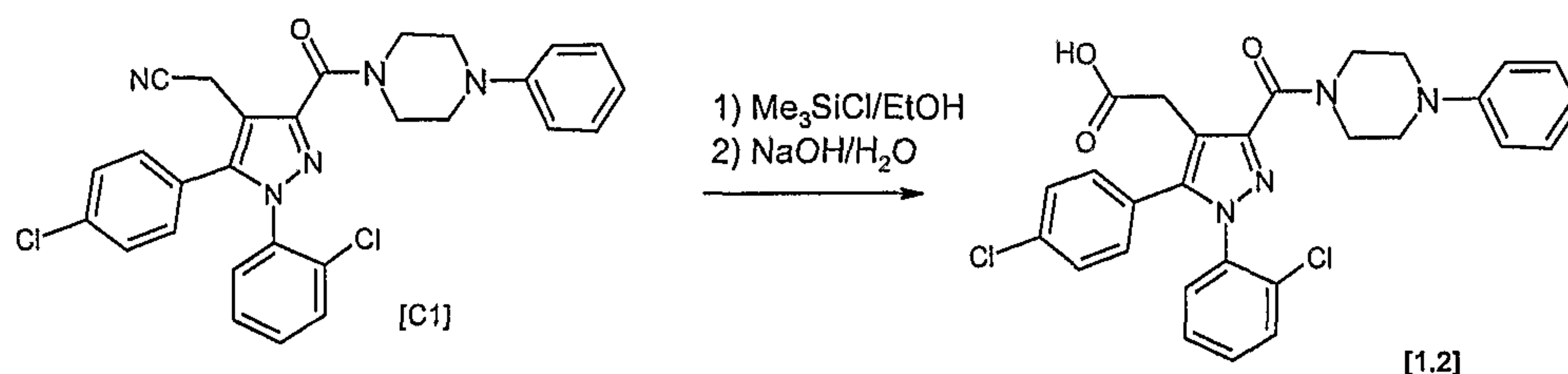
Scheme 8
