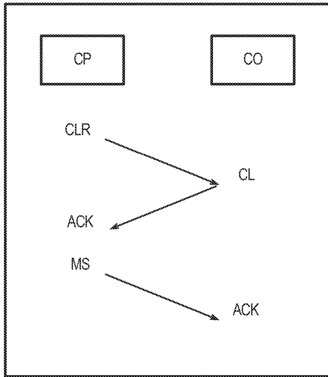
"CP decides" sequence based on G.992.3
