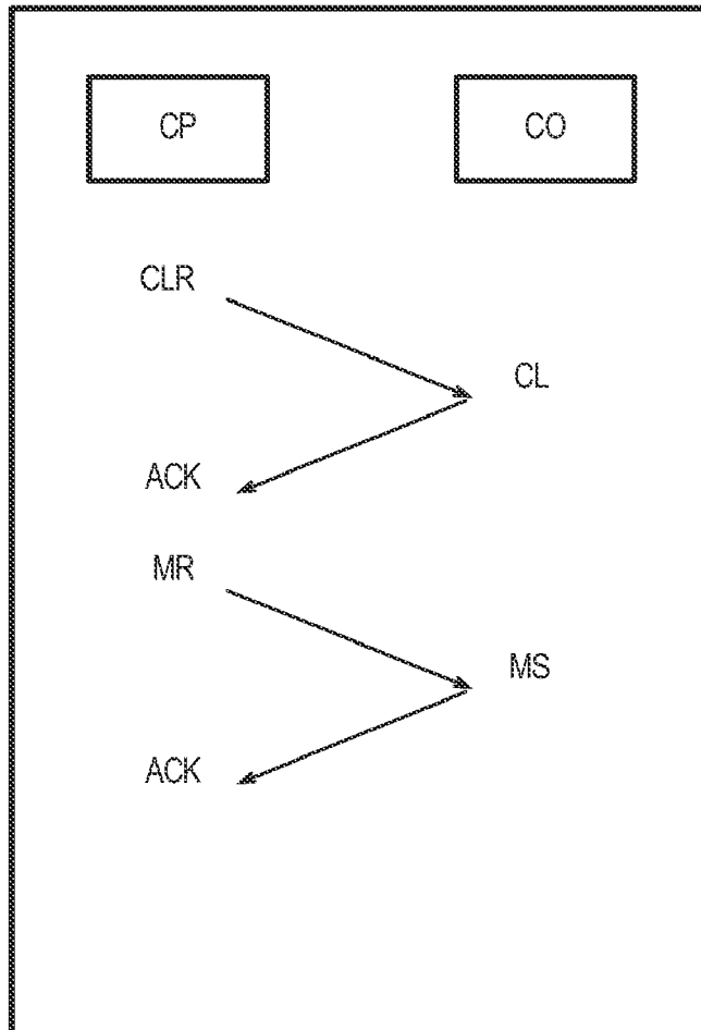
"CO decides" sequence based on G.992.3
