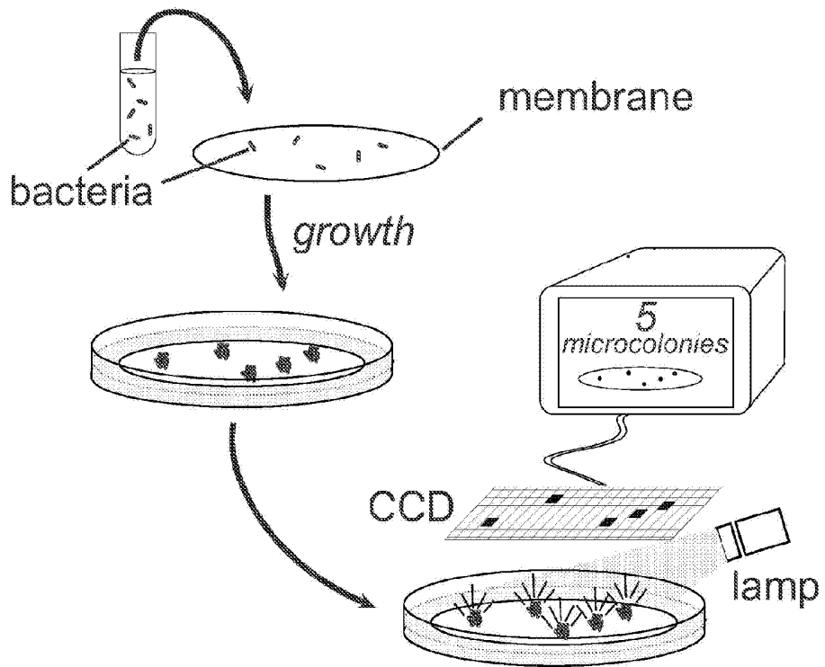
Figure 5. Scheme for reagent-less detection of microcolonies using non-magnified large area imaging.
