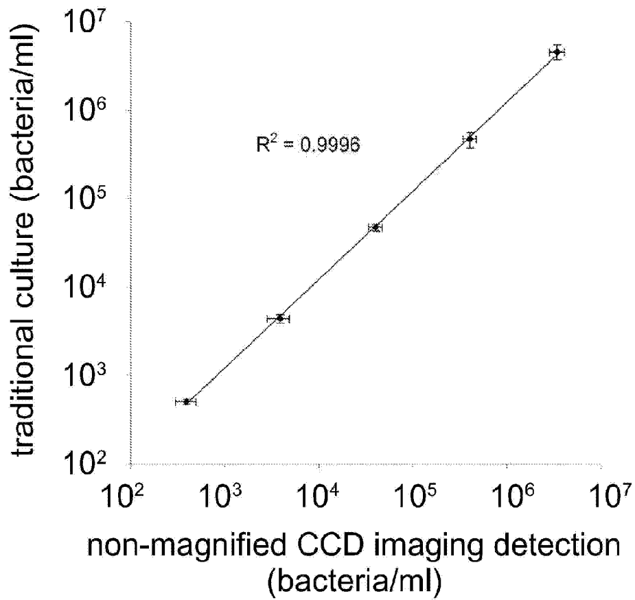
Figure 12. Graph showing correlation between enumeration tests using the invention and traditional culture (Example 7).
