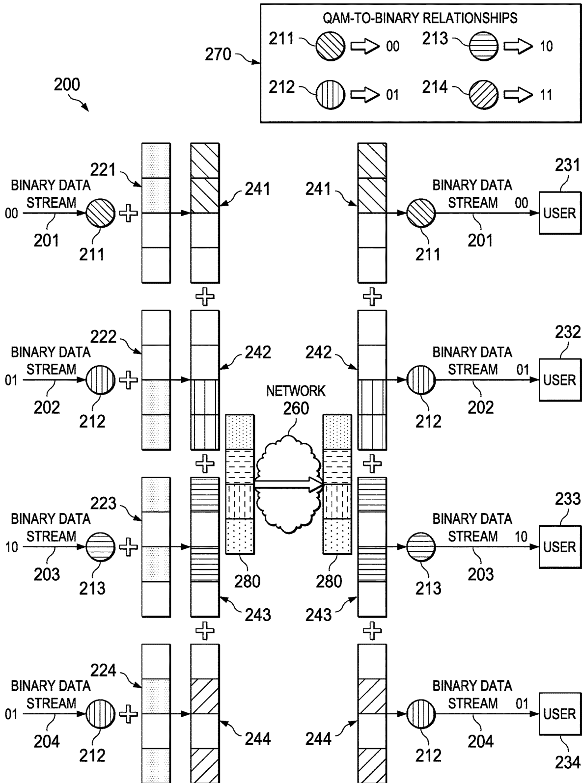
FIG. 2 (PRIOR ART)
