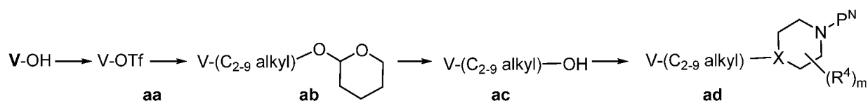
Scheme 7
