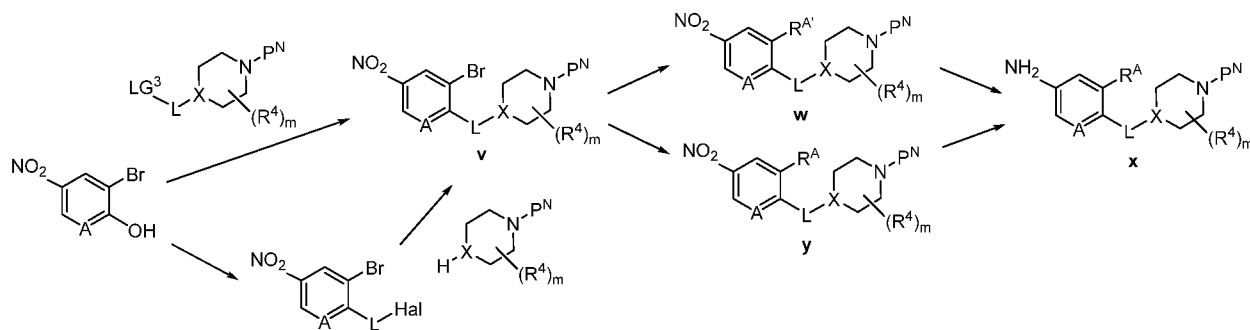
Scheme 6
