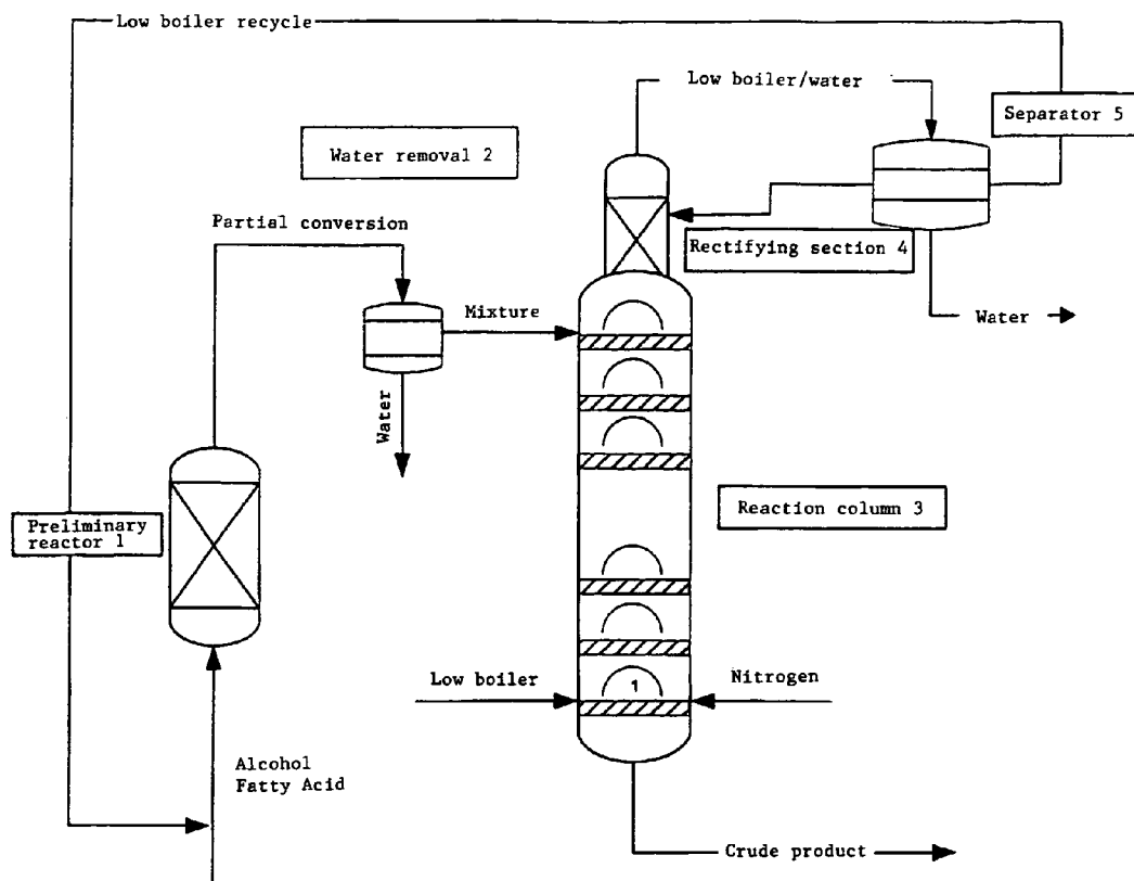
Fig. 1 Process concept for the economic production of long-chain fatty acid esters
