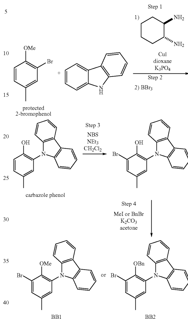
Scheme A1(a): Cross Coupling with Carbazole Derivatives
