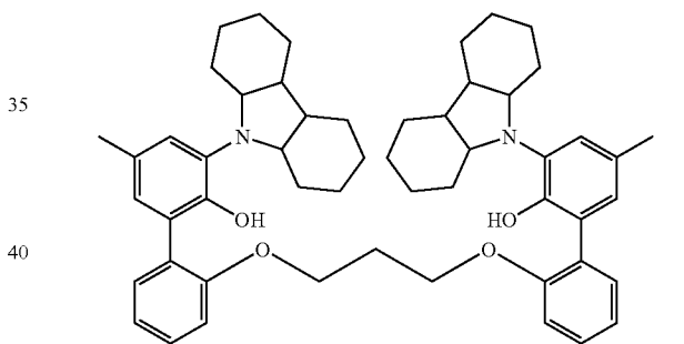
Scheme B2: Synthesis of (O,O)-Bridged Ligand via Upper Phenyl Ring/ Lower Phenyl Ring Double Suzuki or Negishi Cross Coupling Reactions
