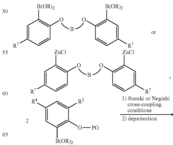
Scheme B2: Synthesis of (O,O)-Bridged Ligand via Upper Phenyl Ring/ Lower Phenyl Ring Double Suzuki or Negishi Cross Coupling Reactions
