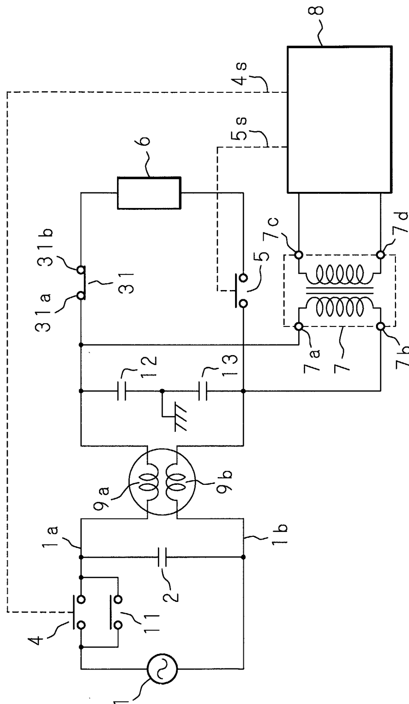
FIG. 2 PRIOR ART
