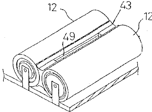
Fig. 11 Prior Art
