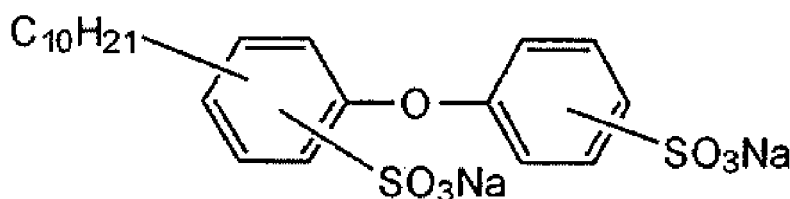
Surfactant-4
