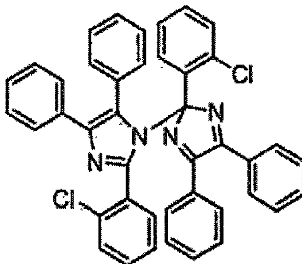
Polymerization initiator (5)
