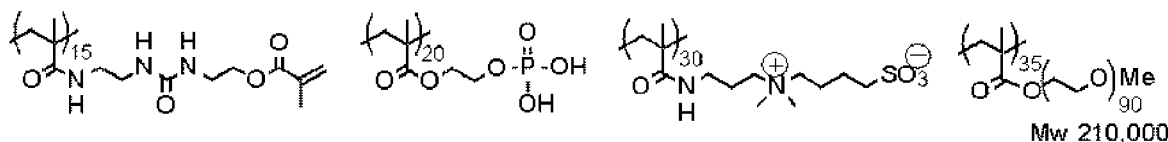
Compound (UC-1) for undercoat layer
