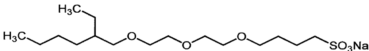
Anionic surfactant 1
