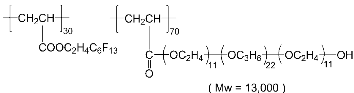
Fluorine-based surfactant (1)
