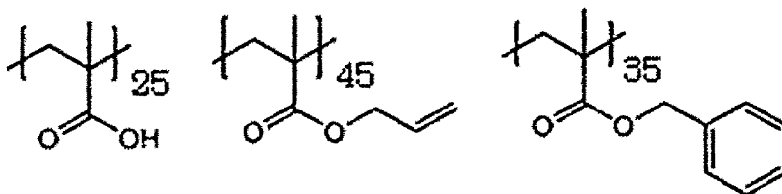
Binder polymer (4)
