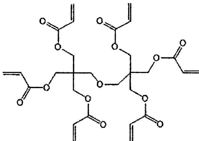
Polymerizable compound (2)
