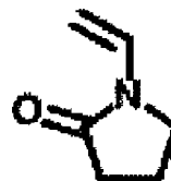
Compound 3
