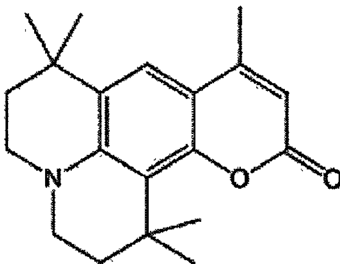
Polymerization initiator (5)
