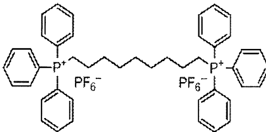
Phosphonium compound (1)
