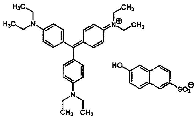
Ethyl violet
