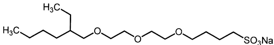
Anionic surfactant 1
