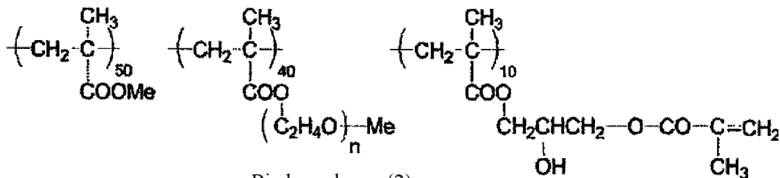
Binder polymer (2)
