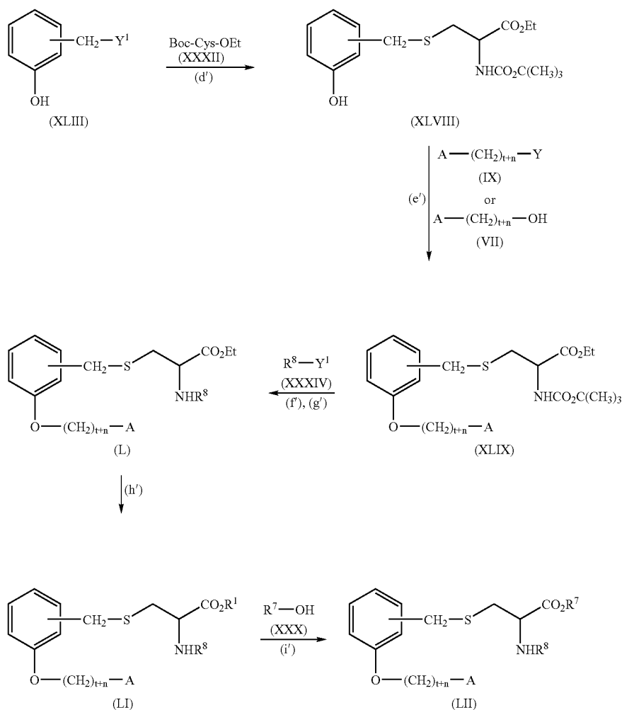
Scheme 17
