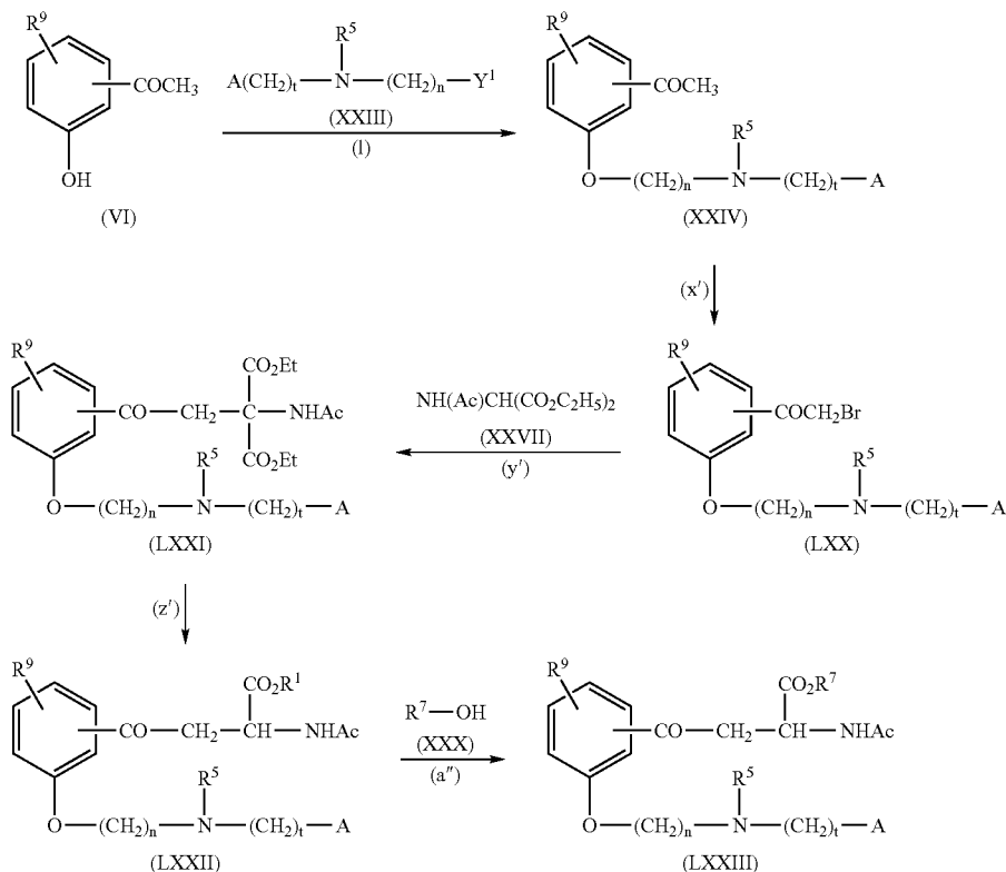
Scheme 8
