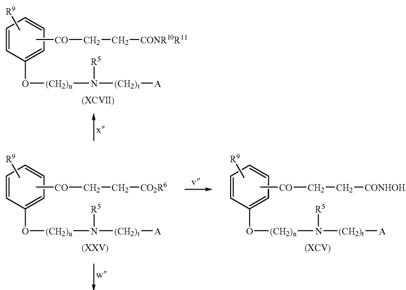
Scheme 22
