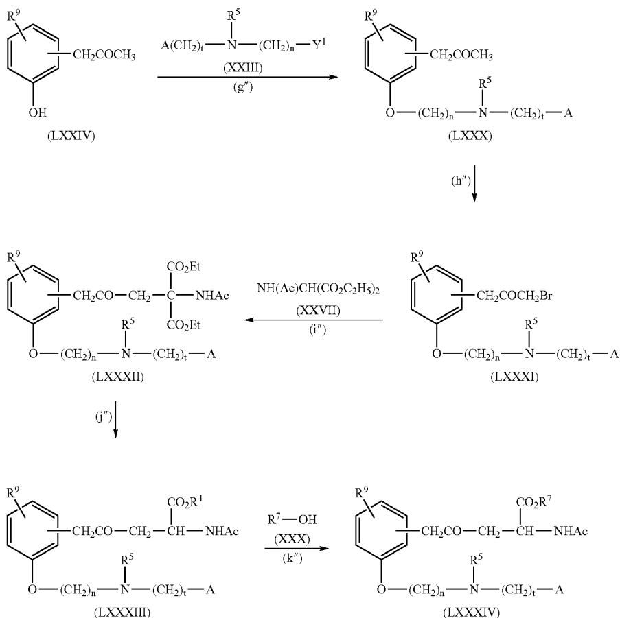
Scheme 10
