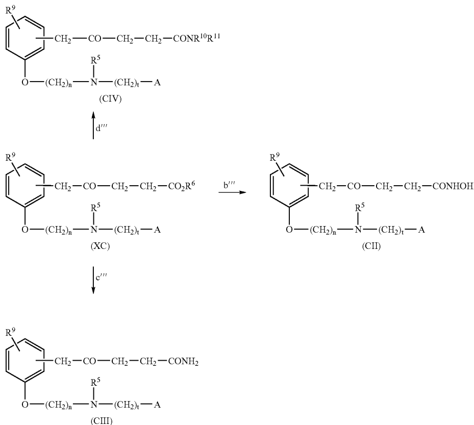
Scheme 24
