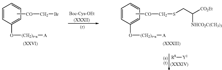
Scheme 14
