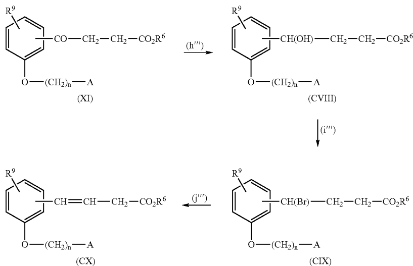
Scheme 27
