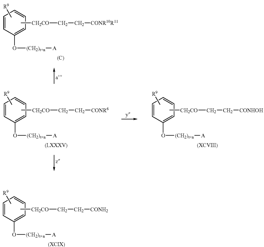
Scheme 23
