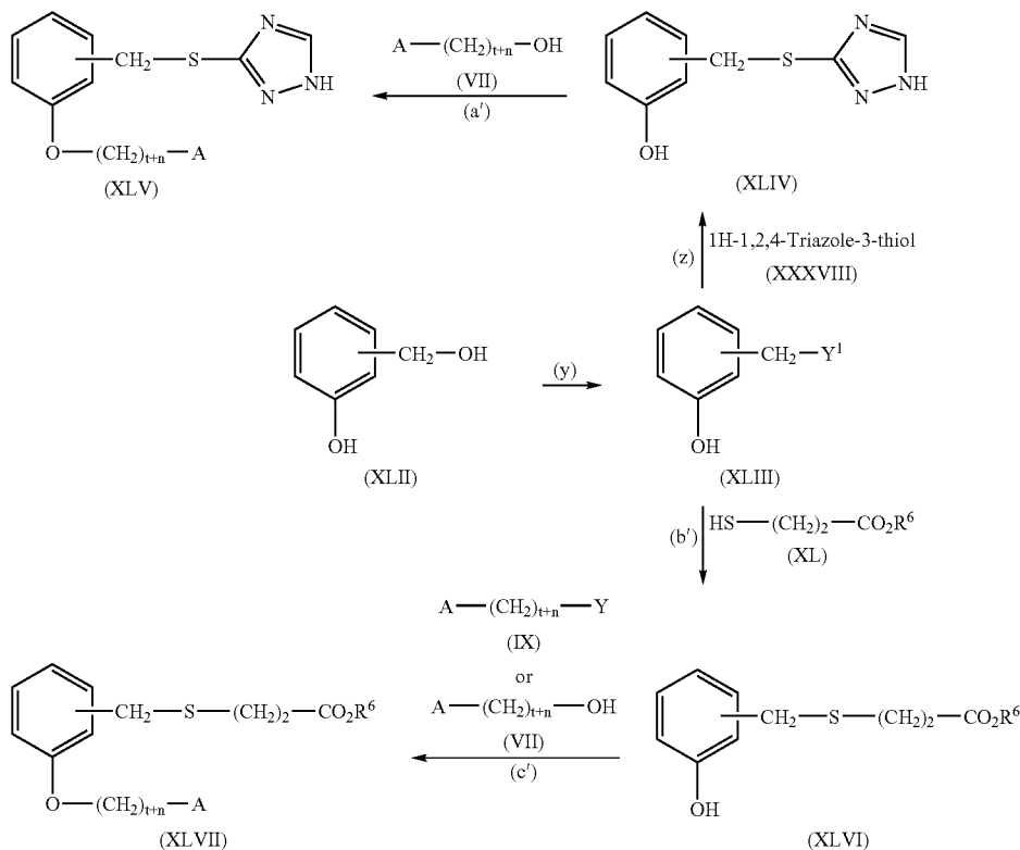
Scheme 16
