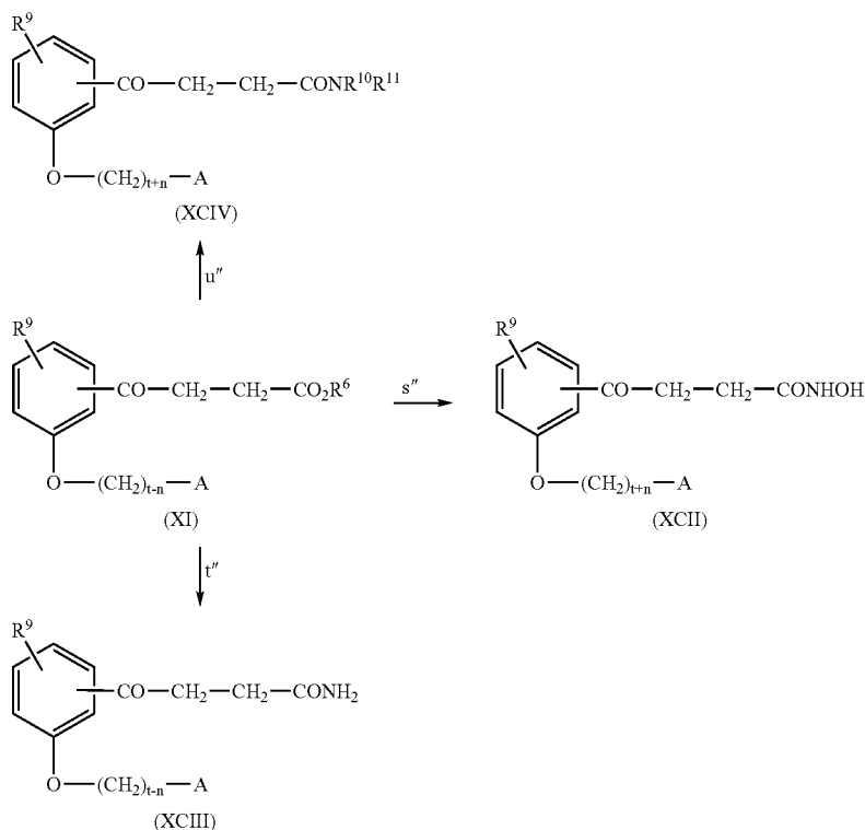
Scheme 21
