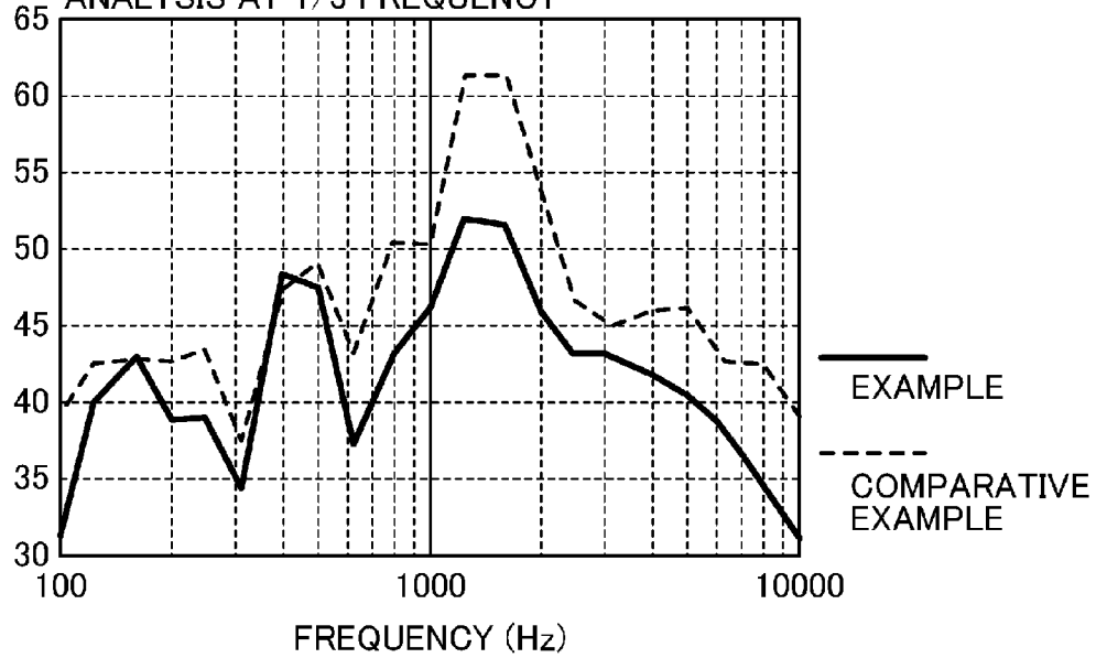
FIG. 13 SOUND PRESSURE (db) GRAPH SHOWING IN COMPARISON RESULTS OF ANALYSIS AT 1/3 FREQUENCY
