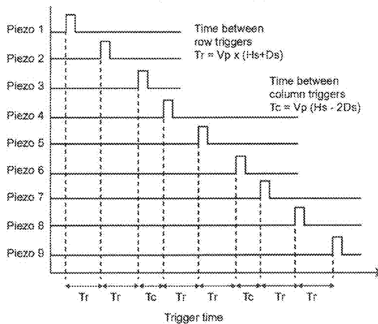
Timing diagram of dispense trigger sequence
