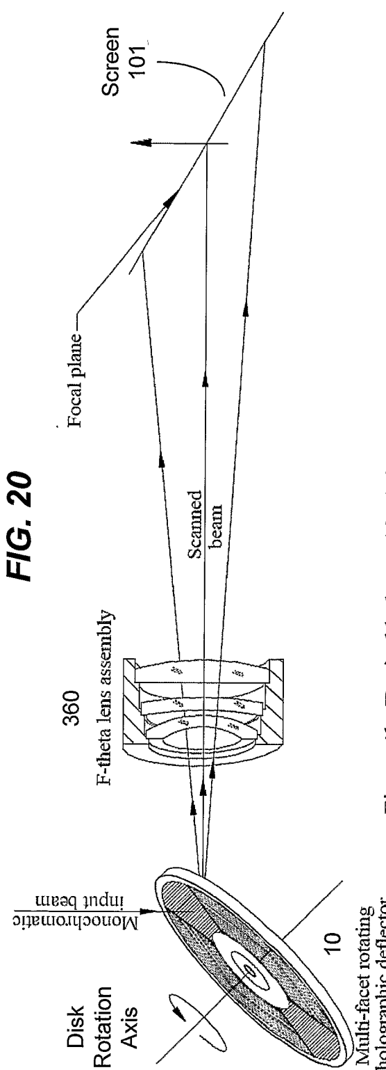
Figure 1b: Typical holographic deflector-based scanner design.
