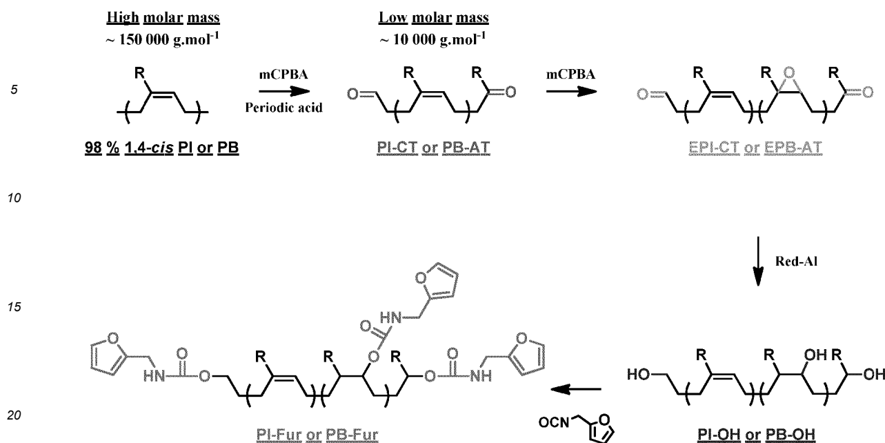
Scheme 1: General synthetic route used for the synthesis of 1,4-cis low molar mass PI-Fur and PB-Fur.
