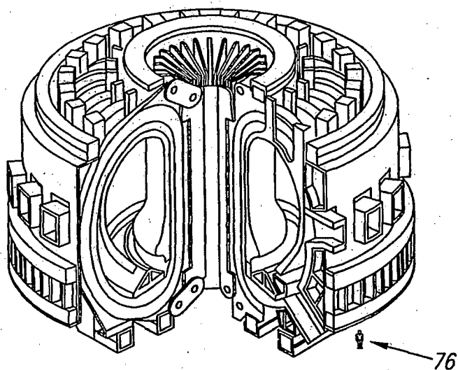
FIG. 7 (PRIOR ART)
