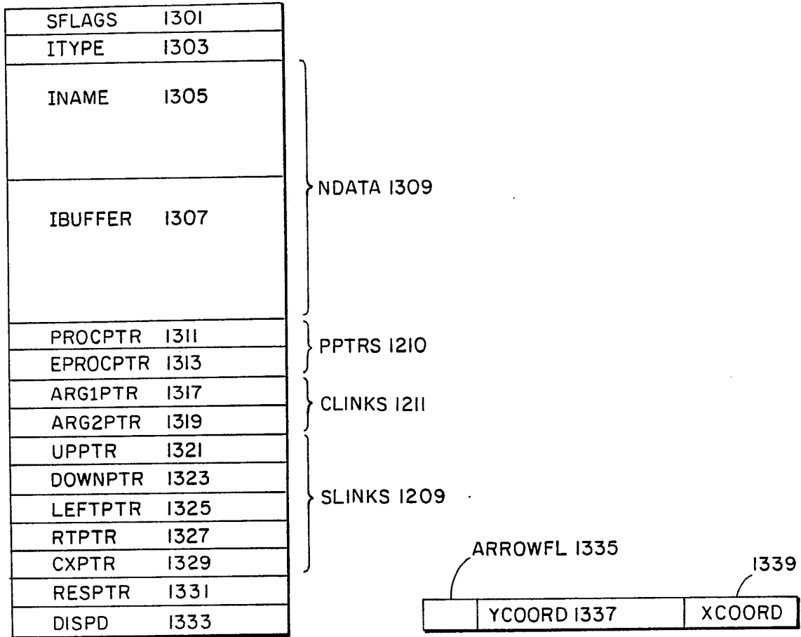
FIG. 13: DETAIL OF NODE 1203
