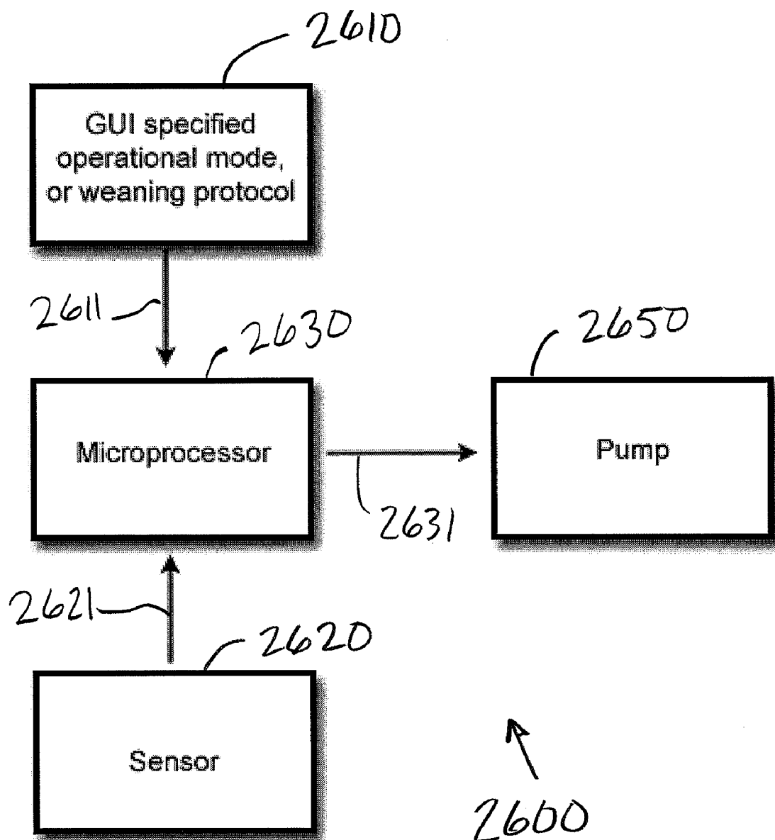
Block diagram of the control scheme.
