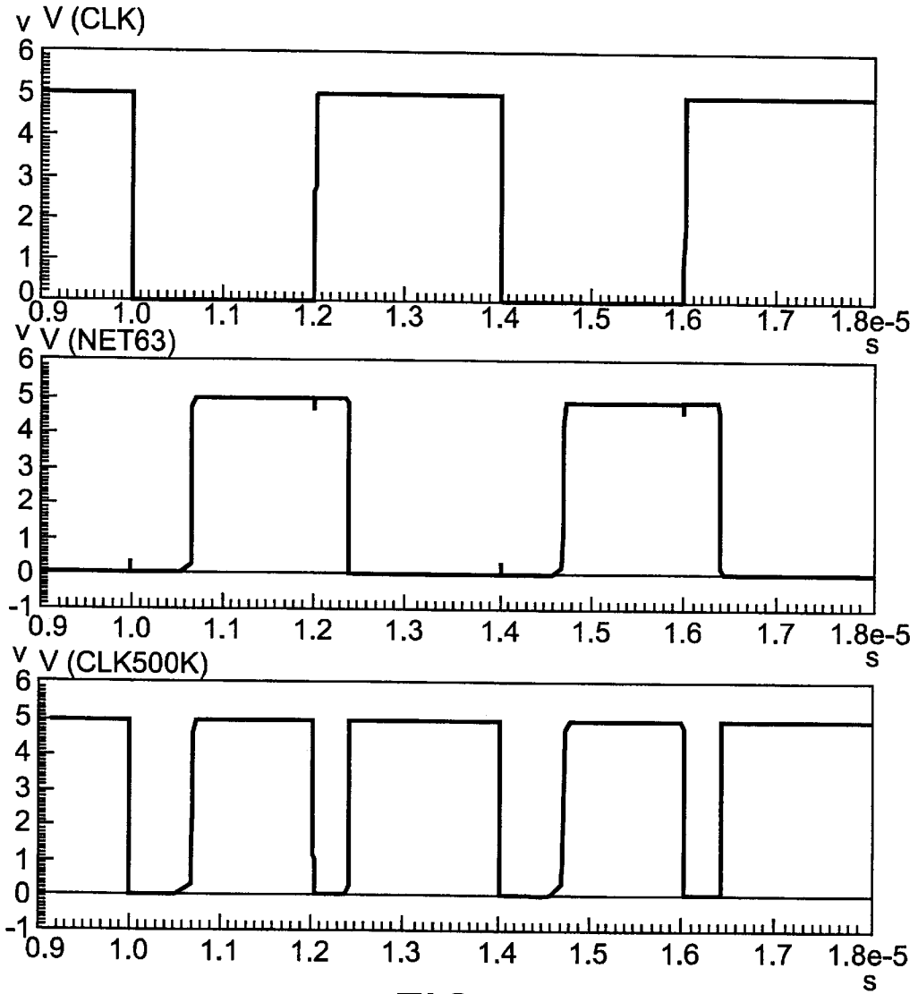
FIG. 2. (PRIOR ART)
