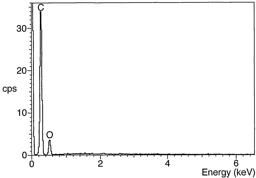
LTC Polymer/PSi/Composite; Polymer only; 20keV
