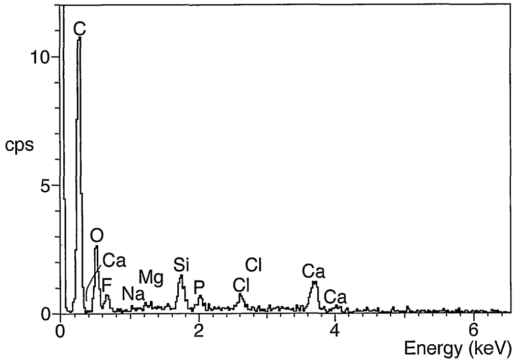
LTC Polymer/PSi/Composite; Hole in HA layer; 20keV
