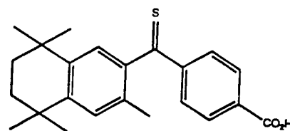
thioketone
