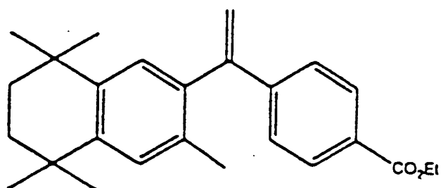
Ethyl-4-[1-(3,5,5,8,8-pentamethyl-5,6,7,8-tetrahydro-2-naphthyl)ethenyl] benzoate
