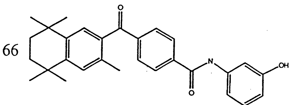
4-[(3,5,5,8,8-pentamethyl-5,6,7,8-tetrahydro-2-naphthyl)carbonyl]-N-(3-hydroxyphenyl)benzamide (3-Me-m-TTNCHBP)
