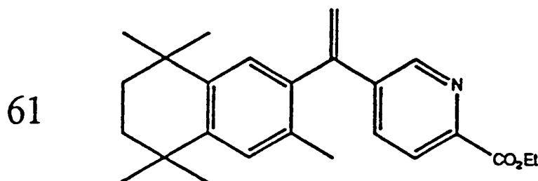
Ethyl-5-[1-(3,5,5,8,8-pentamethyl-5,6,7,8-tetrahydro-2-naphthyl)ethenyl]pyridine-2-carboxylate (3TNEPE)
