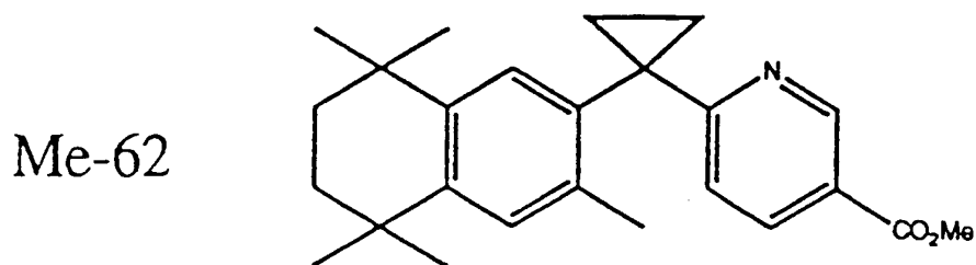
Methyl 2-[1-(3,5,5,8,8-pentamethyl-5,6,7,8-tetrahydro-2-naphthyl)cyclopropyl]pyridine-5-carboxylate
