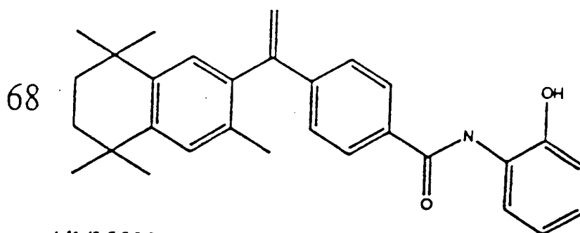
4-[1-(3,5,5,8,8-pentamethyl-5,6,7,8-tetrahydro-2-naphthyl)ethenyl]-N-(2-hydroxyphenyl)benzamide (3-Me-o-TTNCBHP)
