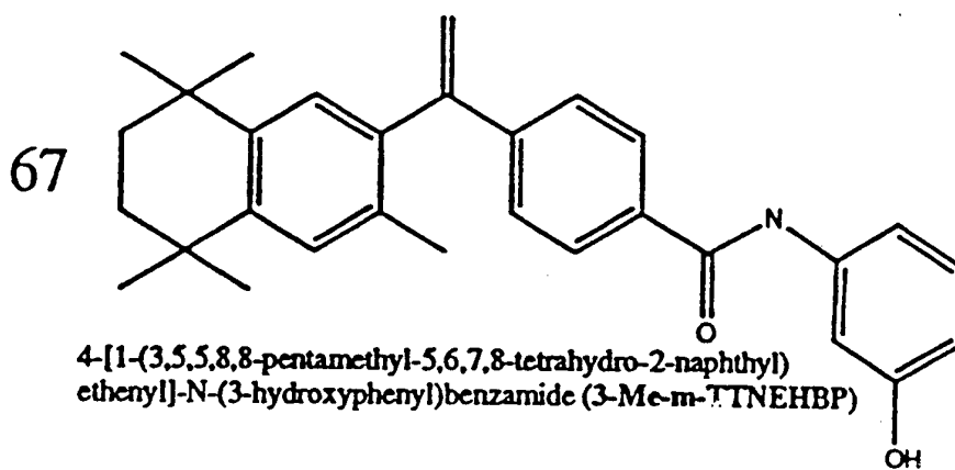
4-[(3,5,5,8,8-pentamethyl-5,6,7,8-tetrahydro-2-naphthyl)carbonyl]-N-(3-hydroxyphenyl)benzamide (3-Me-m-TTNCHBP)
