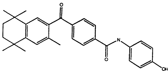
3-methyl-TTNCHBP
